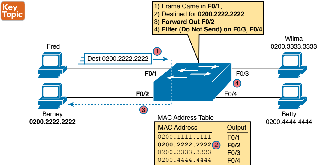
Figure 5-3 Sample Switch Forwarding and Filtering Decision
