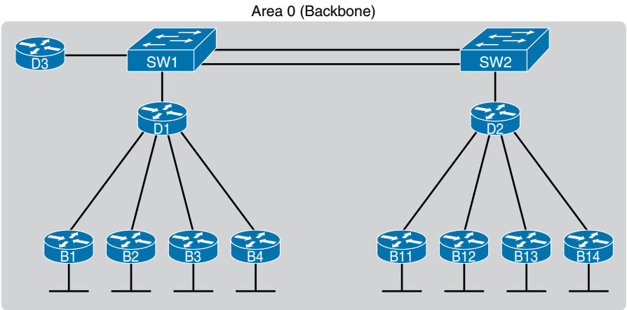
Figure 19-12 Single-Area OSPF
