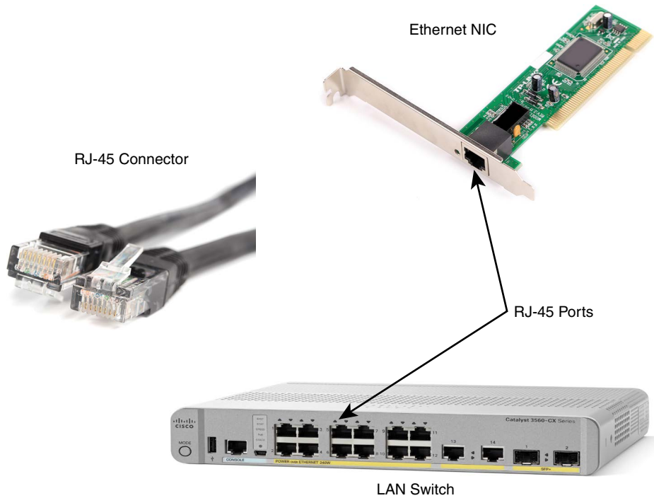
Figure 2-7 RJ-45 Connectors and Ports (Ethernet NIC © Oleg Begunenko/123RF, RJ-45 Connector © Anton Samsonov/123RF)
