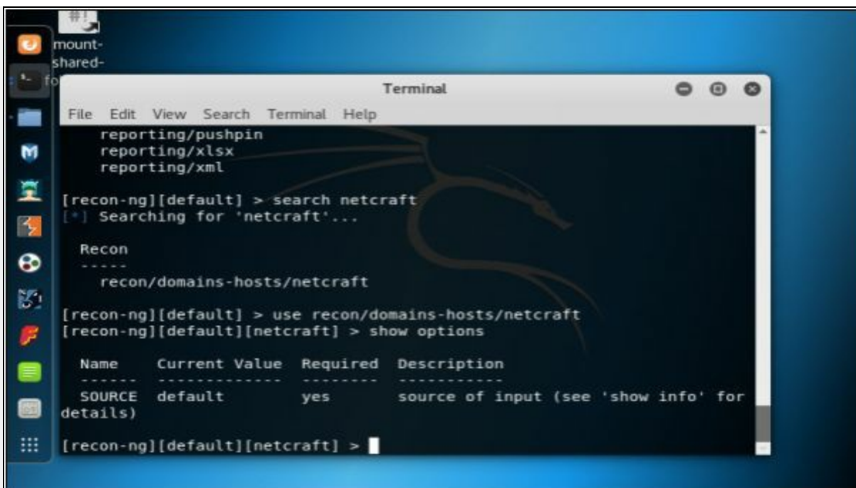
Figure 2-51 Using Netcraft through Recon-ng
