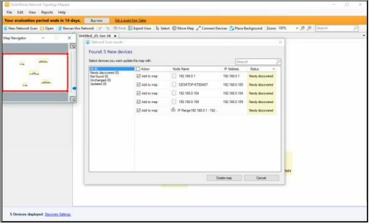
Figure 3-45 Discovered Devices List
