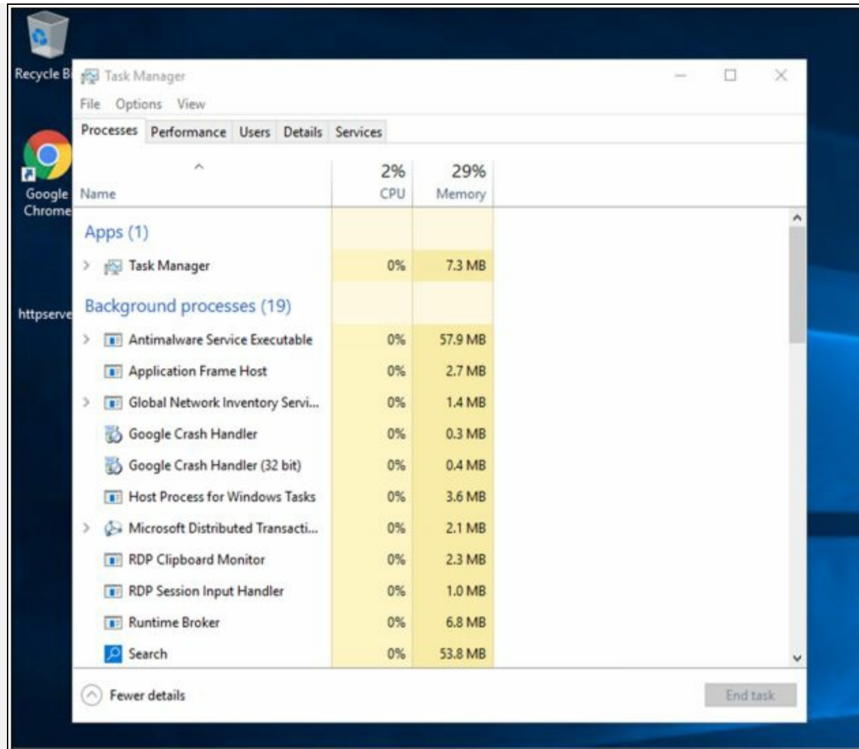
Figure 7-13 Verifying Process
