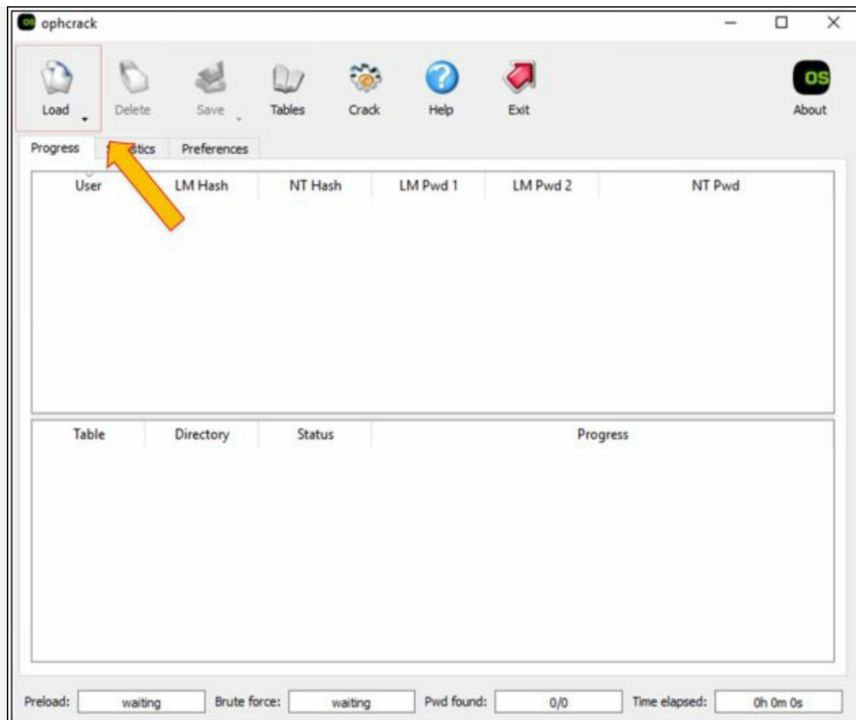
Figure 6-25 Ophcrack tool
