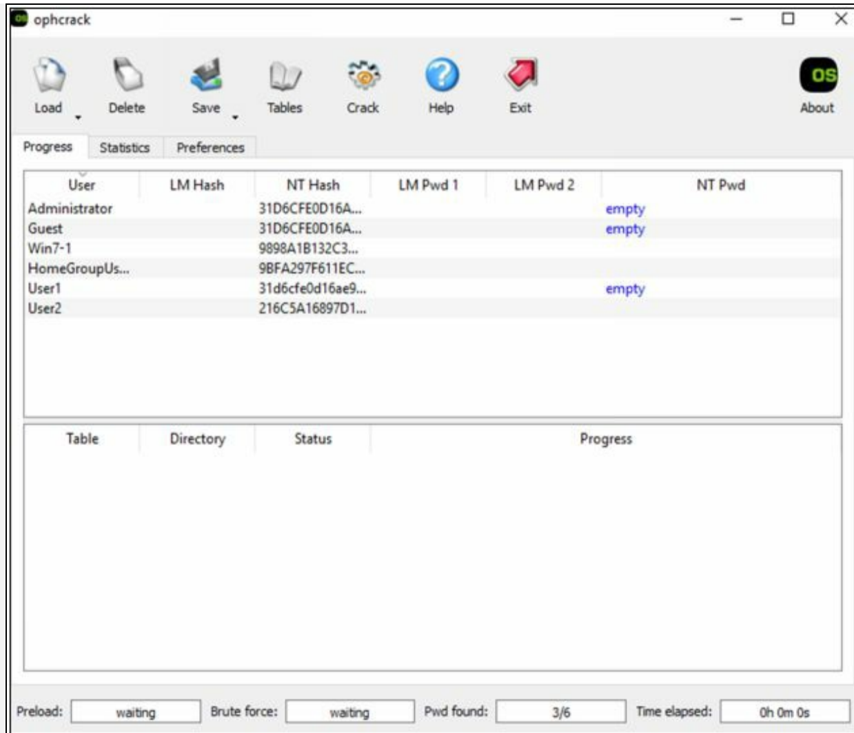
Figure 6-27 File loaded
