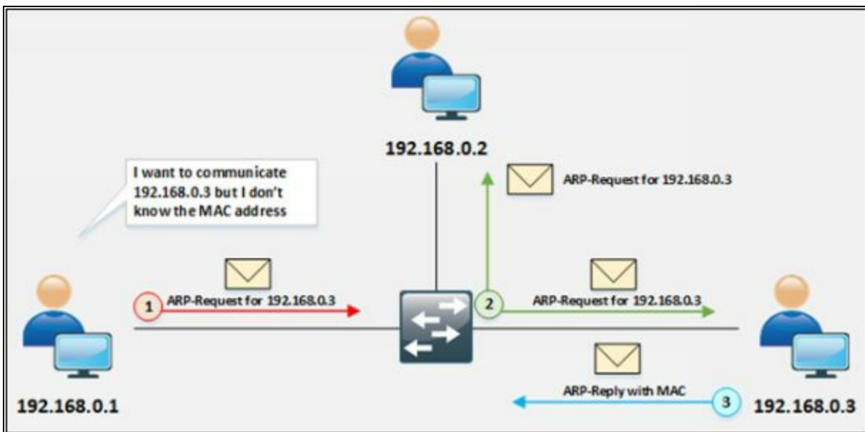
Figure 8-10 ARP Operation
