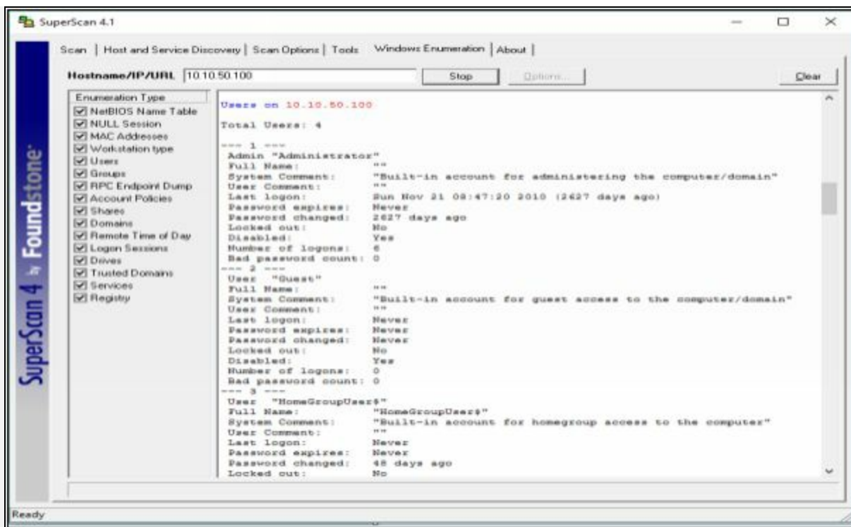
Figure 4-07 Windows Enumeration
