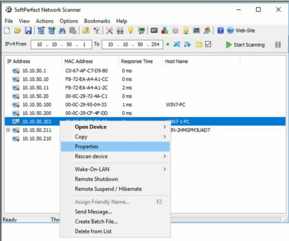
Figure 4-14 Exploring Results
