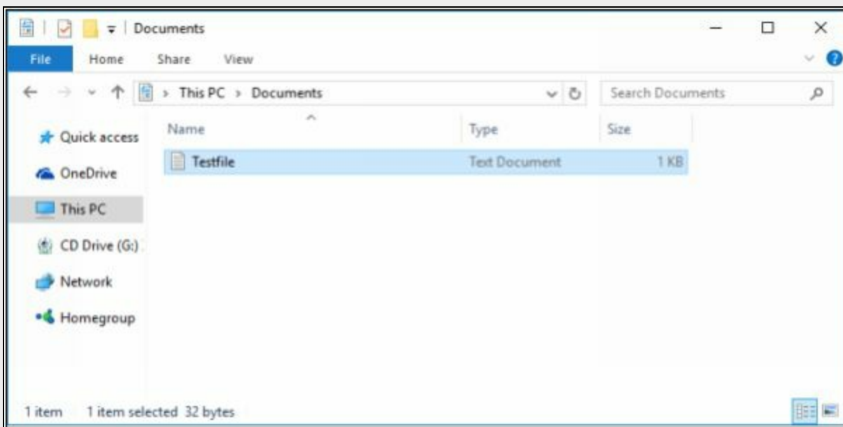
Figure 6-46 File directory
