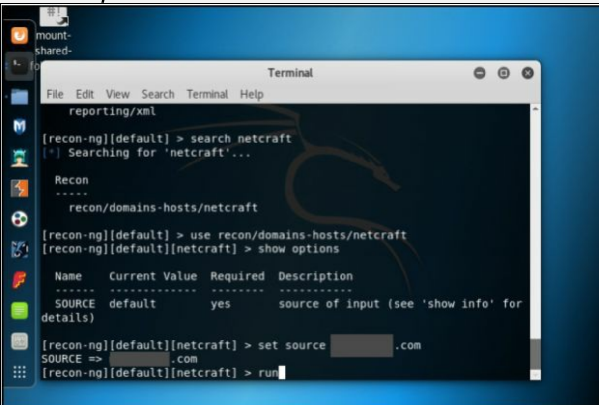
Figure 2-52 Searching for Target Domain
