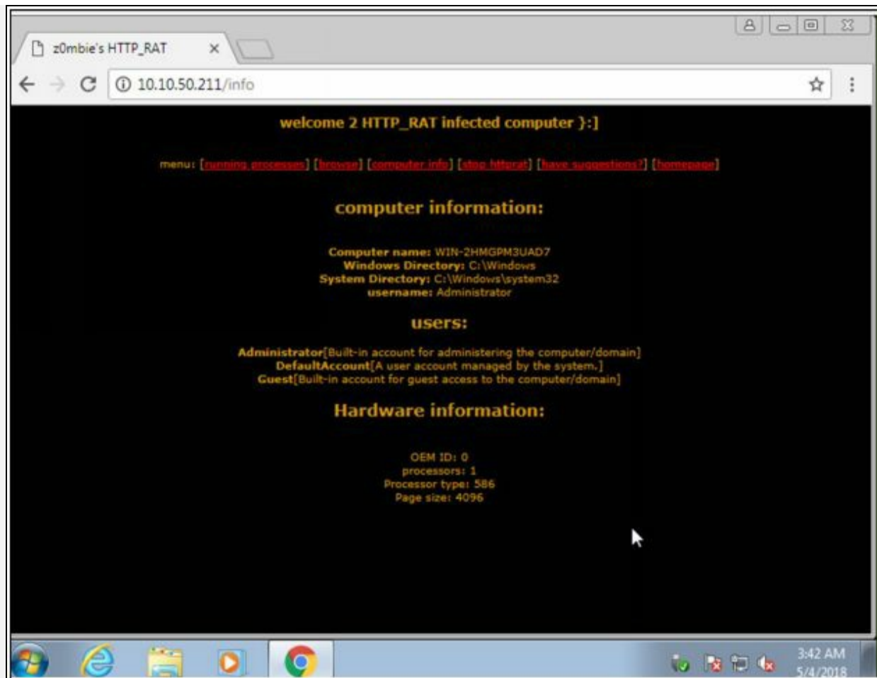
Figure 7-18 HTTP RAT Connection
