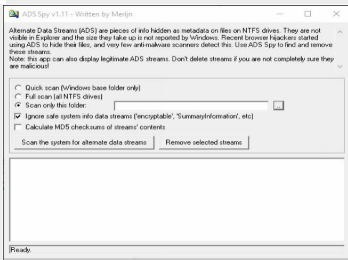
Figure 6-47 ADS Spy Application
