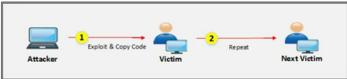
Figure 10-08 Autonomous Propagation
