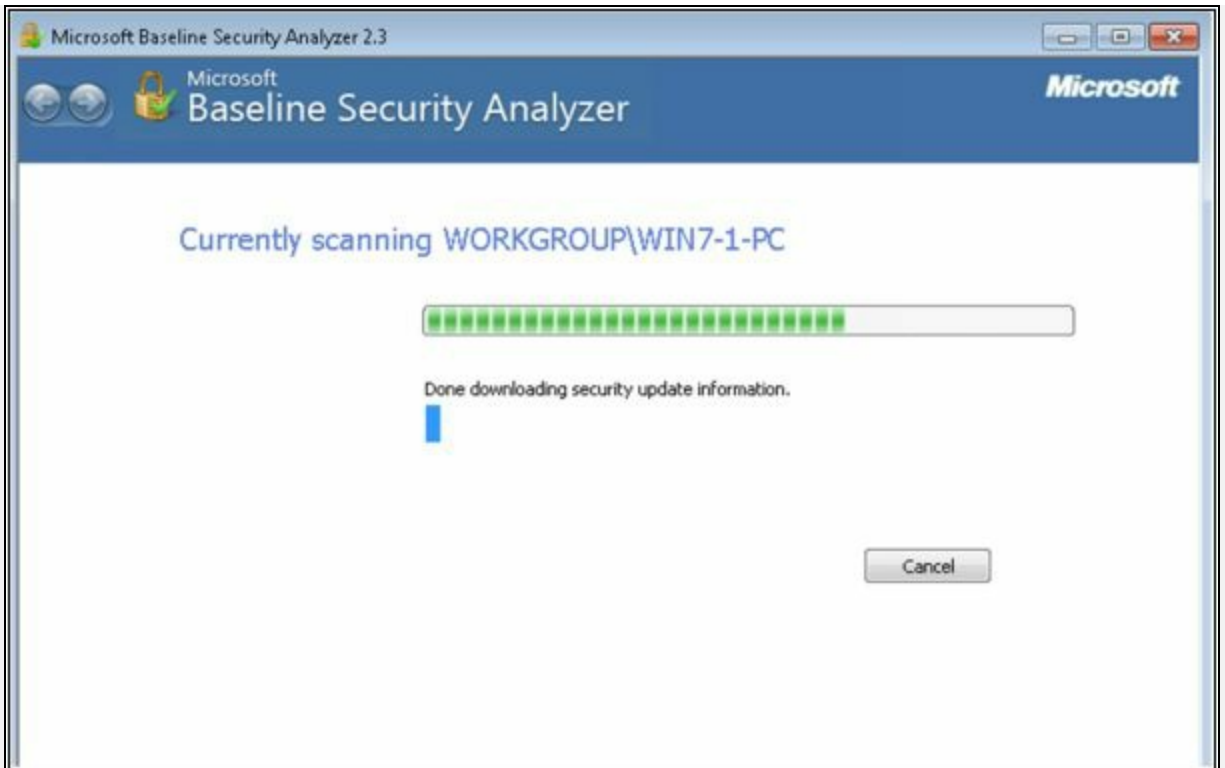
Figure 13-10 MBSA Scanning
