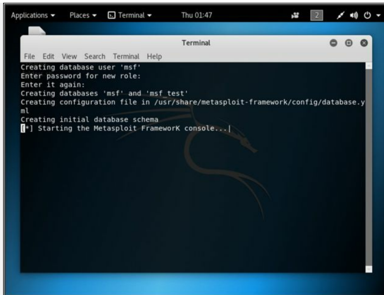
Figure 2-79: Metasploit Framework
