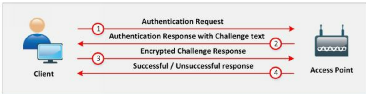
Figure 16-05 Shared Key Authentication
