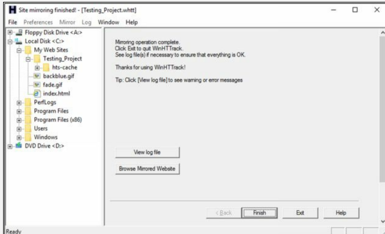
Figure 2-74: Copying complete
