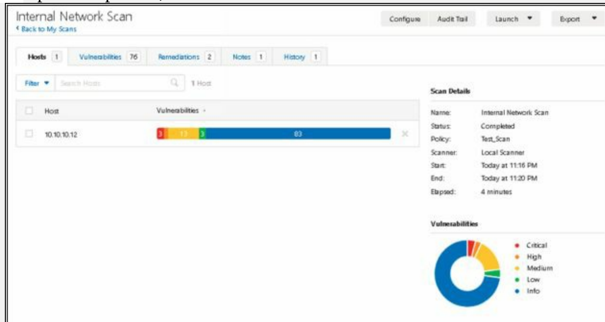
Figure 5-28 Scan results
