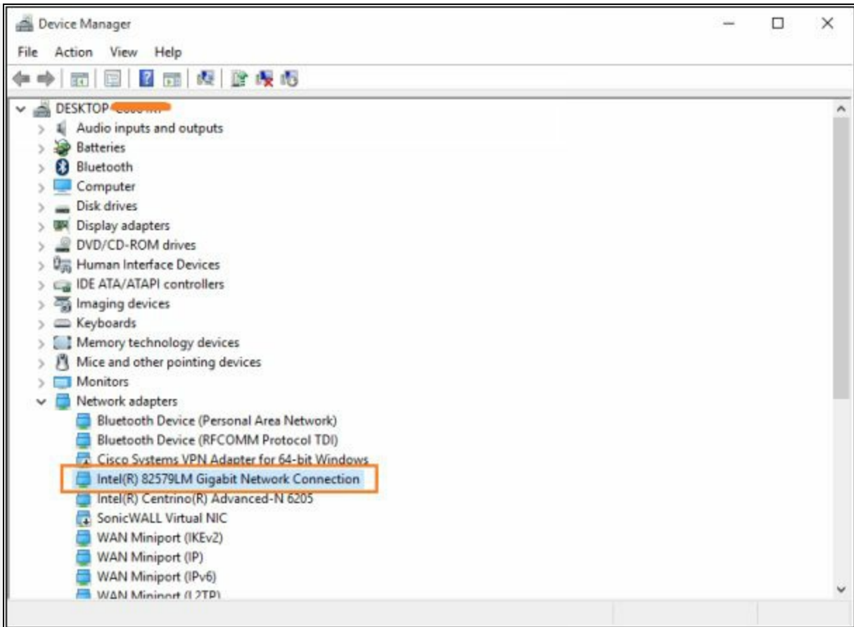
Figure 8-17 Device Manager
