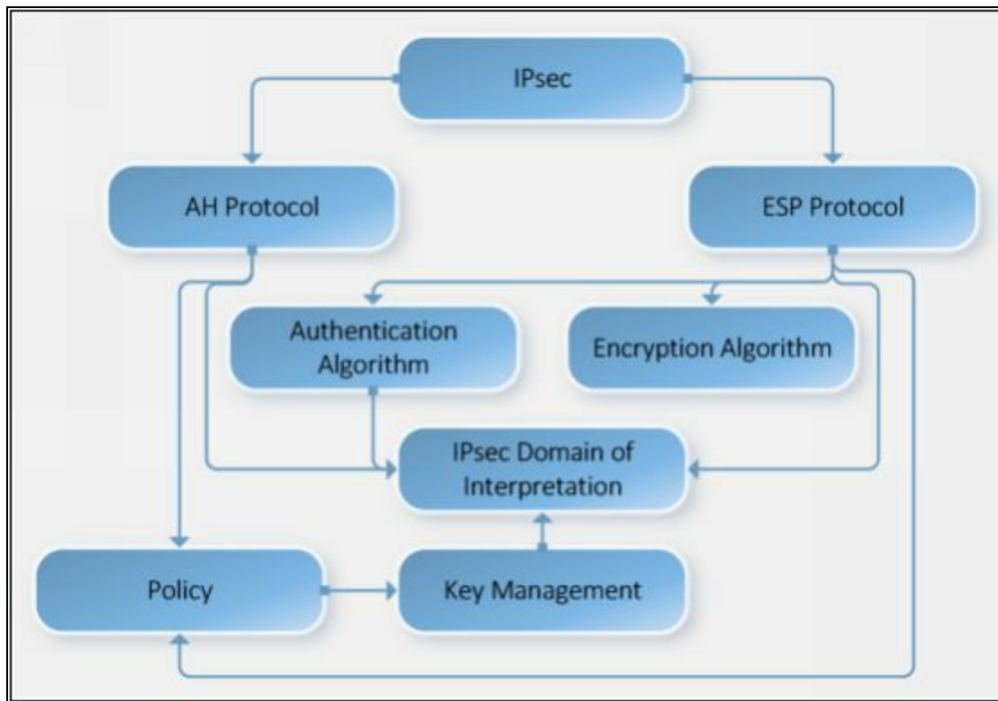
Figure 11-07 IPsec Architecture
