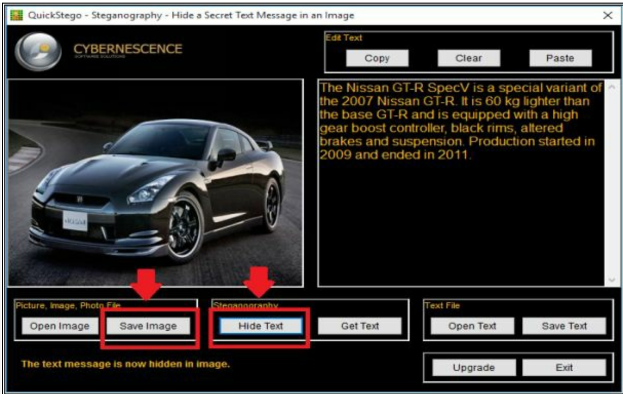
Figure 6-60 Image Steganography
