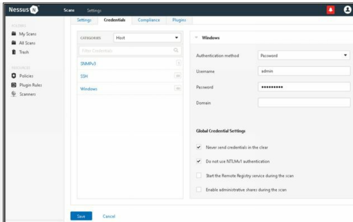
Figure 5-20 Configuring Policy
