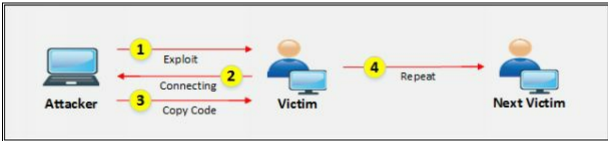
Figure 10-07 Back-Chaining Propagation
