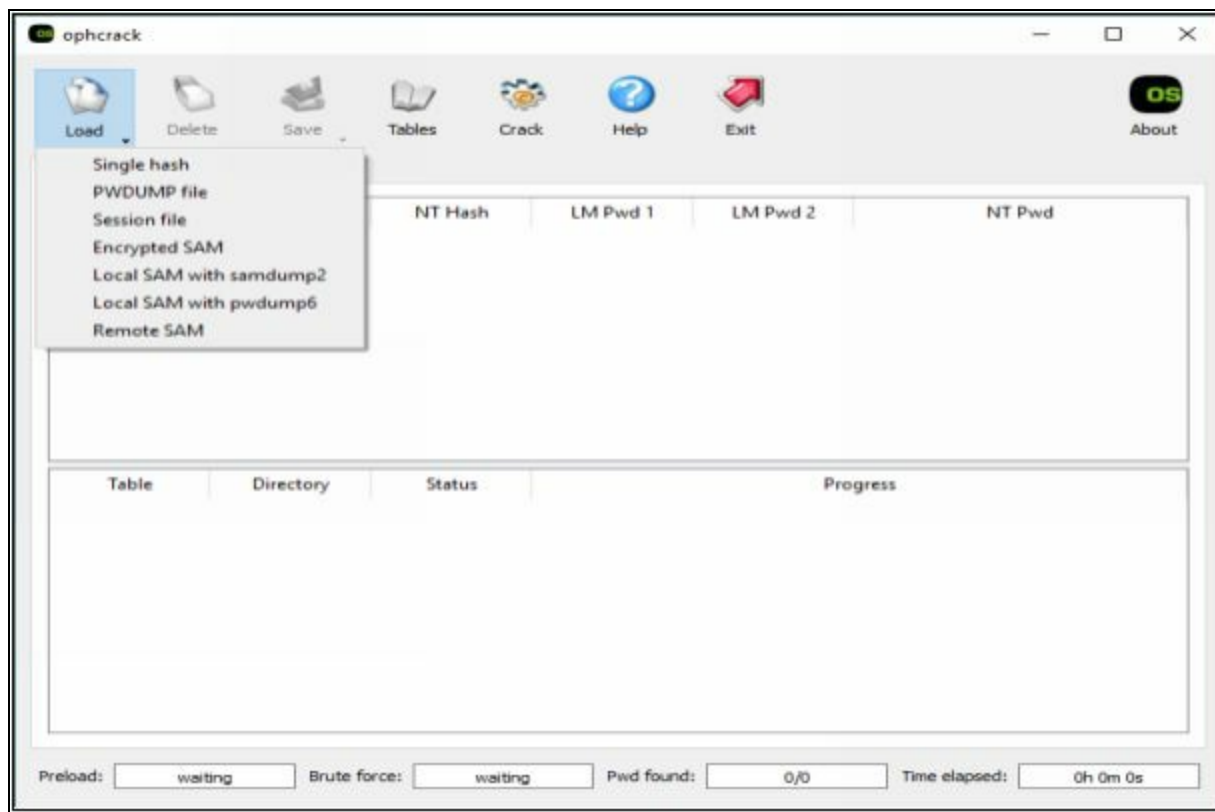
Figure 6-16 Ophcrack Software
