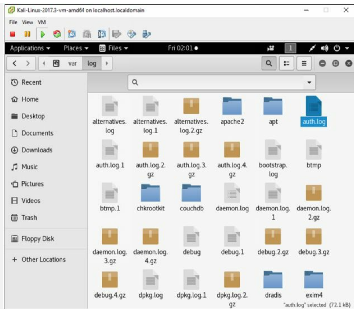
Figure 6-77 /var/log/ directory
