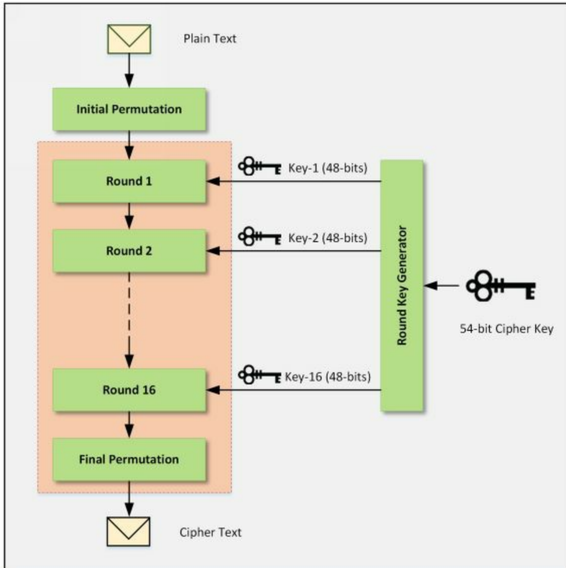
Figure 20-03. DES Algorithm
