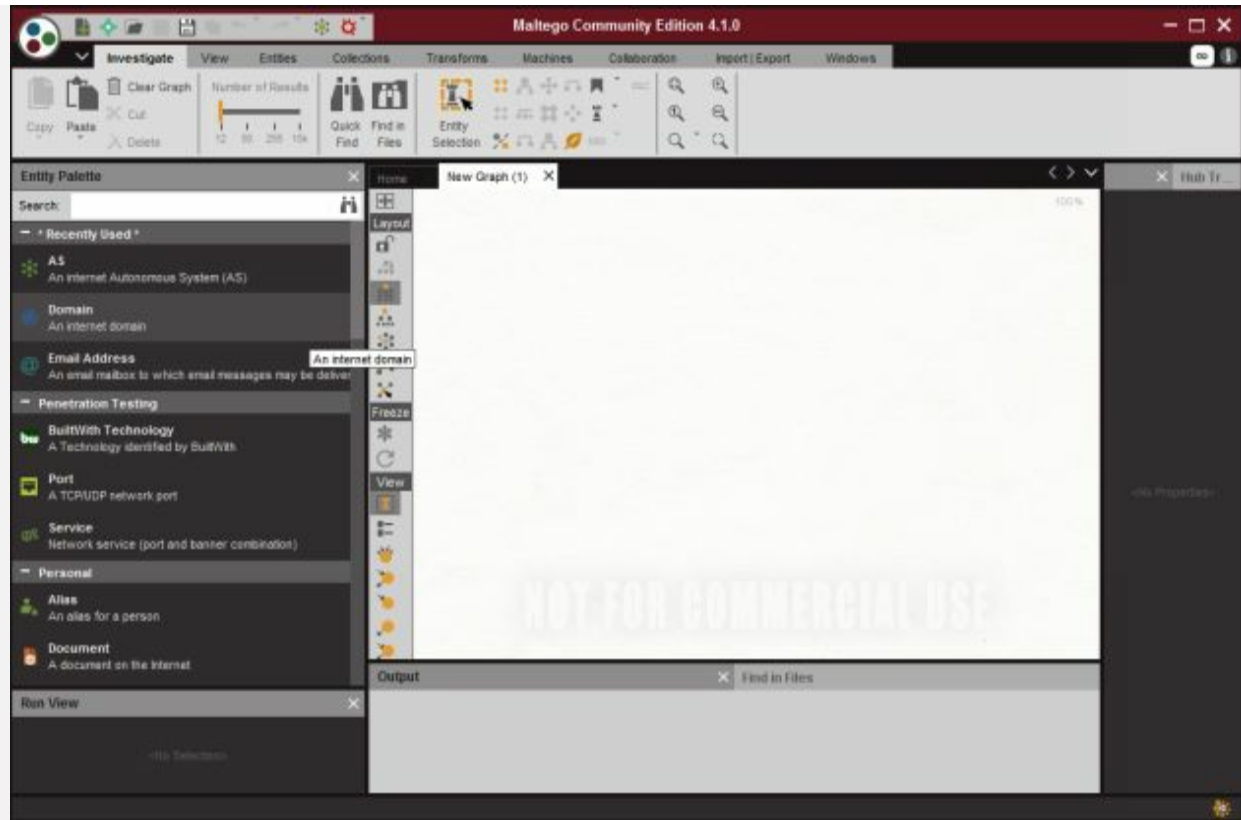
Figure 2-45 Maltego
