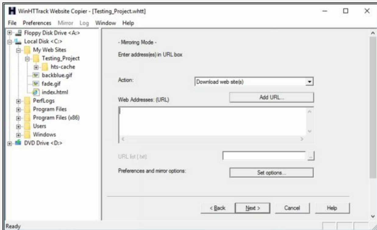
Figure 2-70: Setting Target
