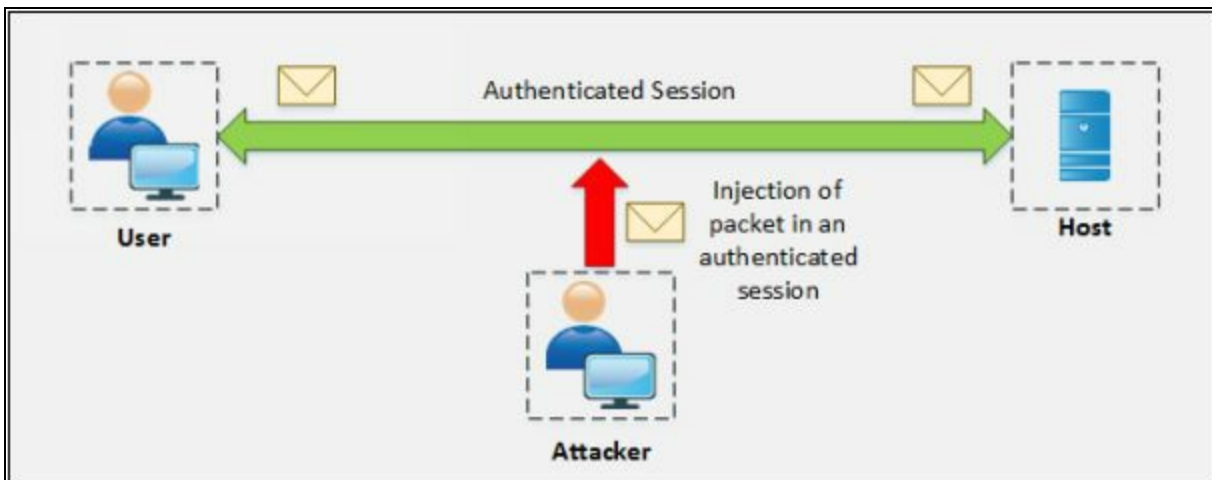
Figure 11-03 Active Attack
