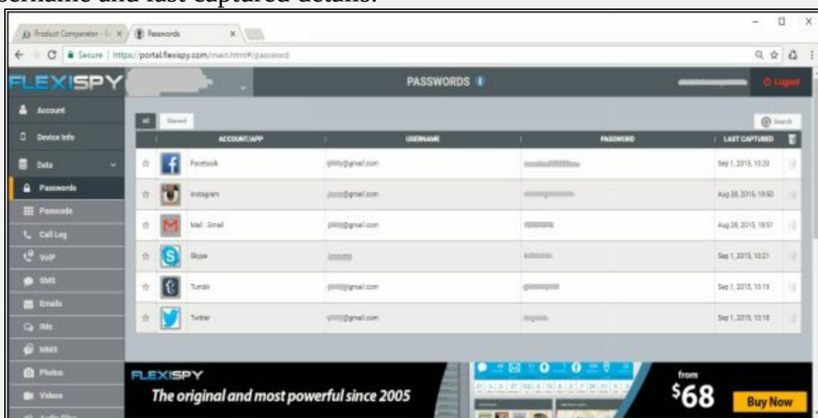
Figure 6-19 FlexySpy
