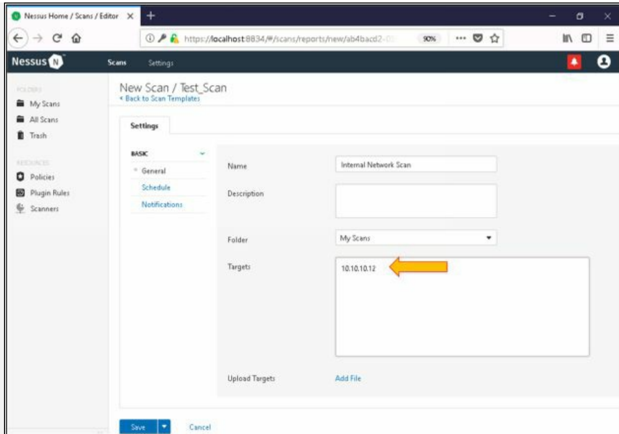
Figure 5-25 Configuring Scan
