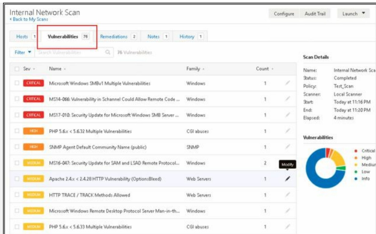
Figure 5-29 Scan results
