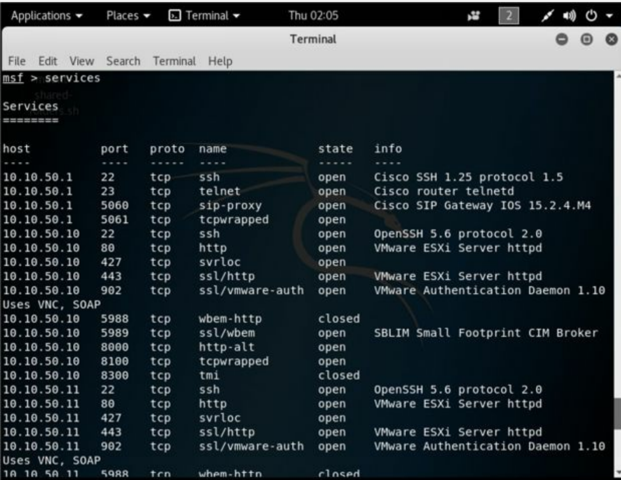
Figure 2-82: Service Scan results
