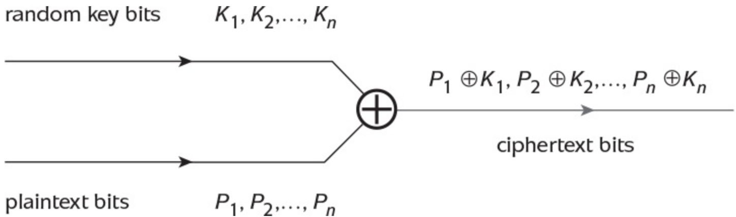
Figure 3.1: The Vernam Cipher.
