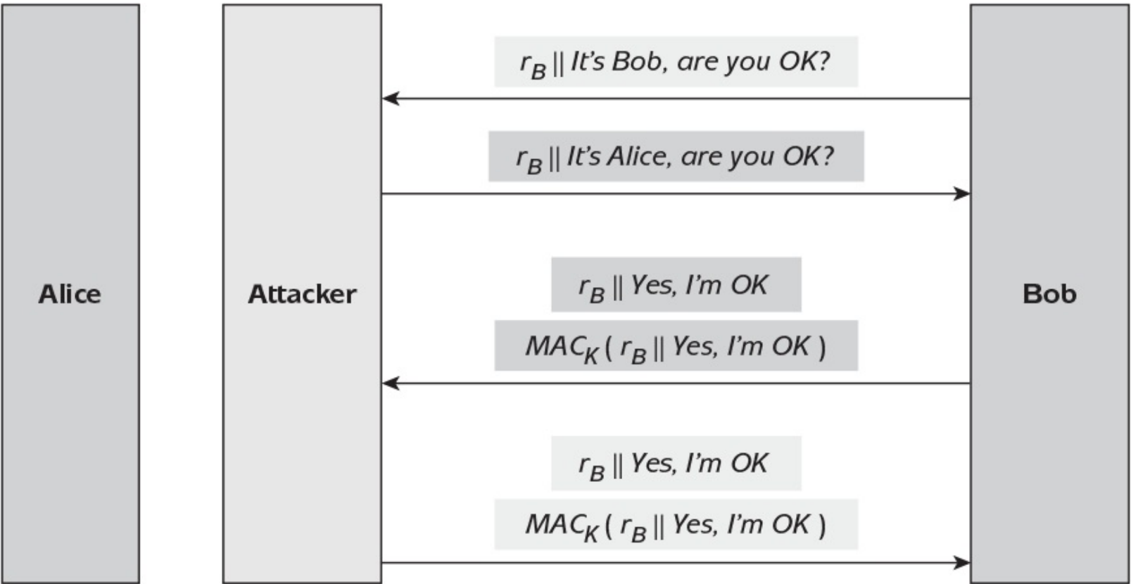
Figure 9.5: Reflection attack against Protocol 3.
