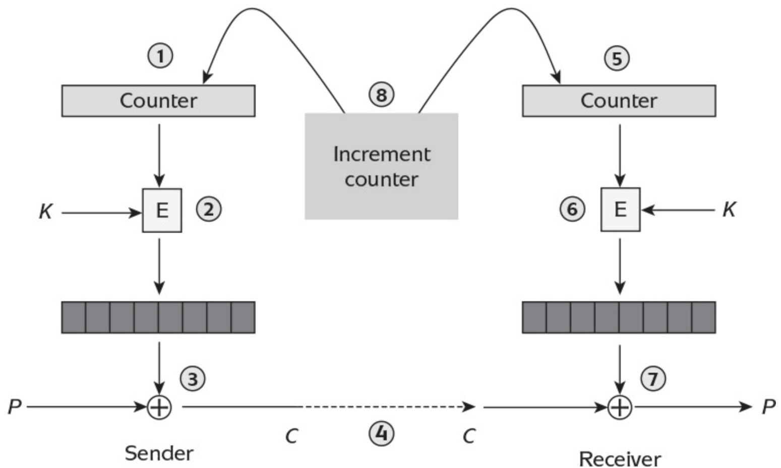
Figure 4.14: Encryption and decryption using CTR mode.
