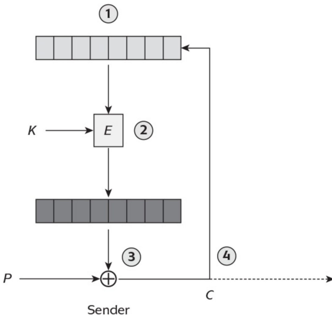
Figure 4.12: Encryption using CFB mode.
