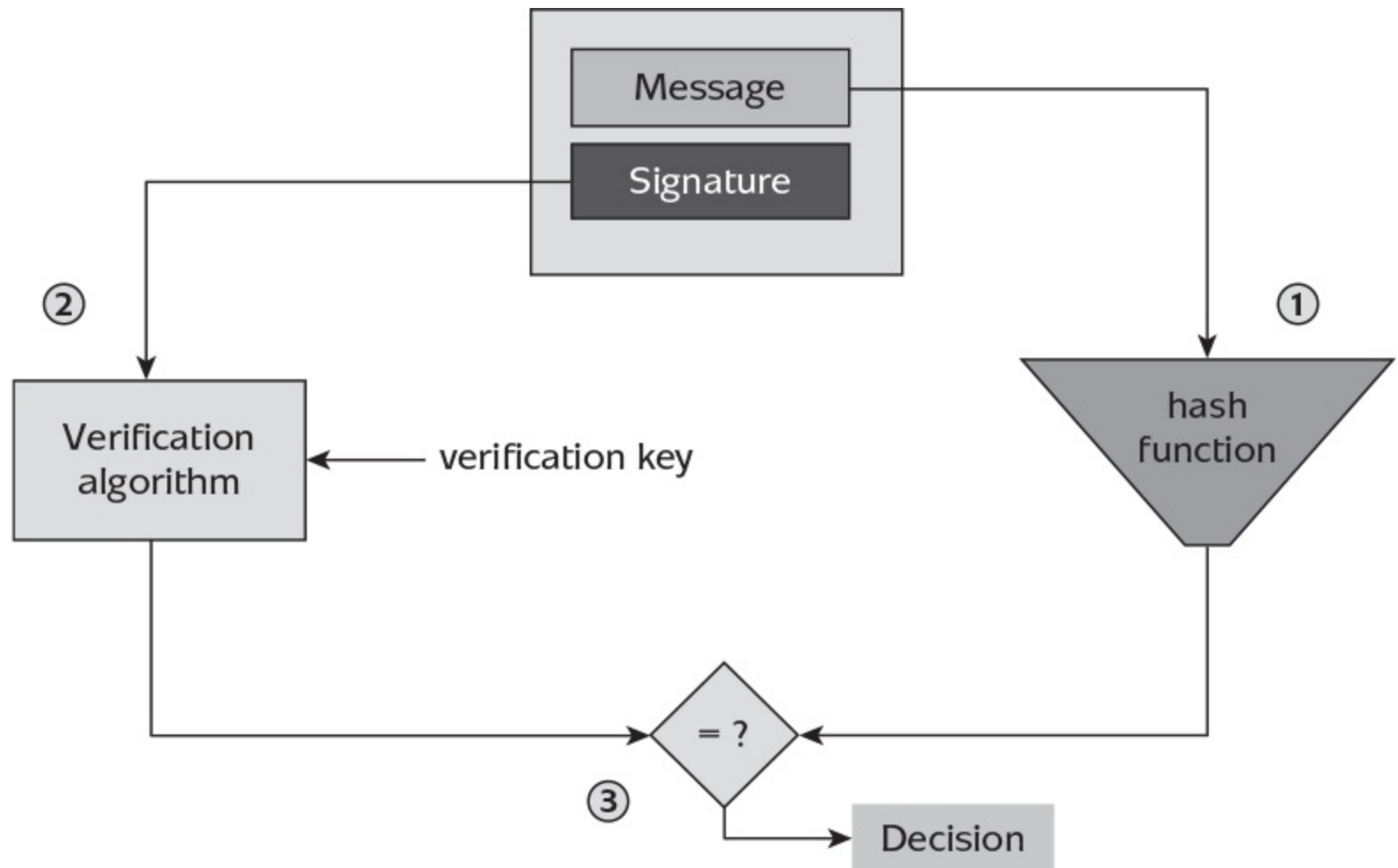
Figure 7.4: Verification of an RSA digital signature with appendix.
