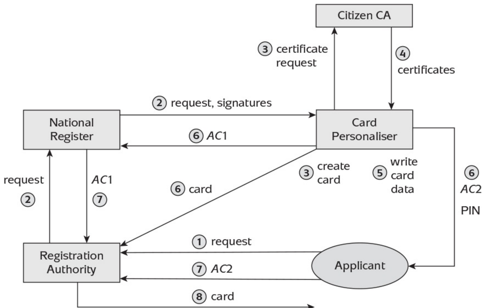
Figure 12.16: eID card issuing process.
