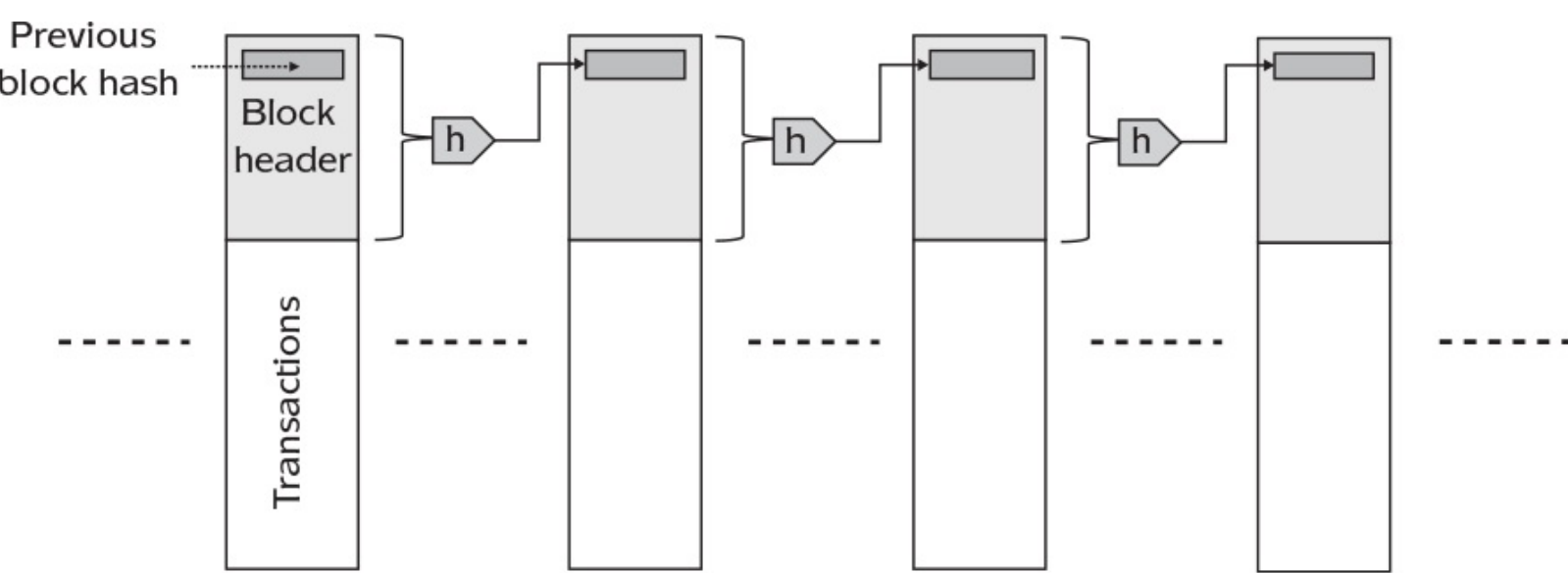
Figure 12.19: The Bitcoin blockchain.
