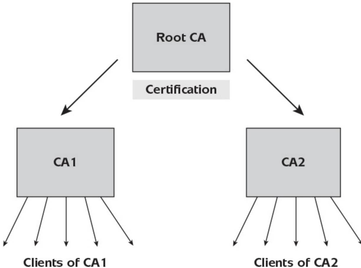
Figure 11.6: Certification hierarchy.
