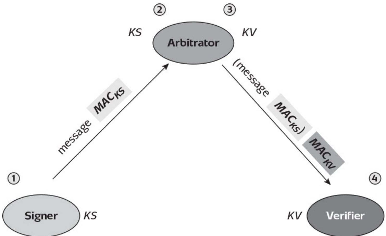
Figure 7.1: An arbitrated digital signature scheme.
