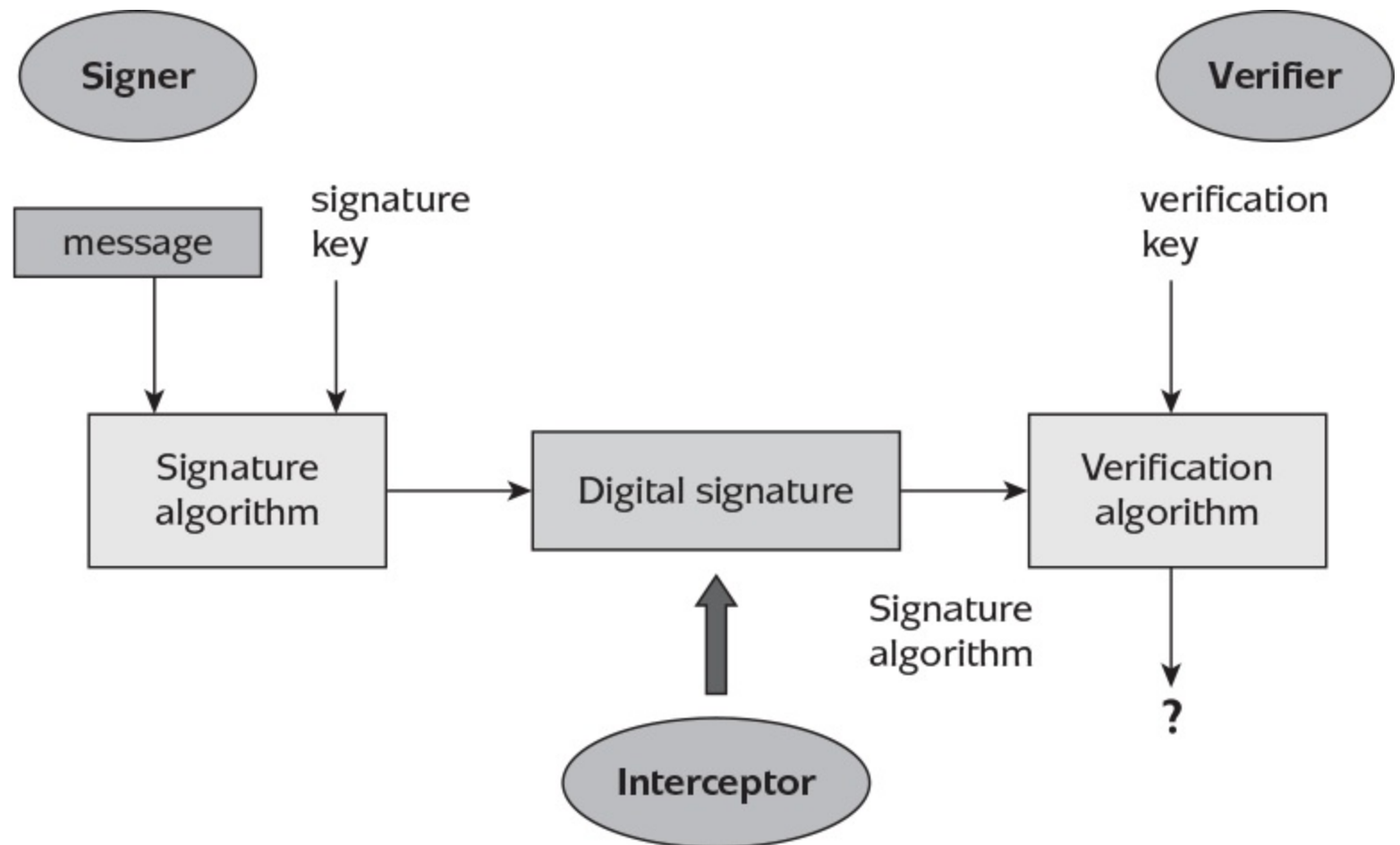
Figure 7.2: Basic model of a digital signature scheme.
