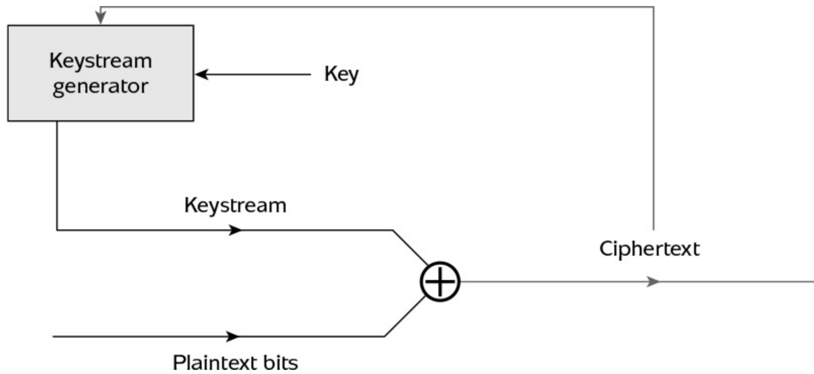
Figure 4.3: Self-synchronising stream cipher.
