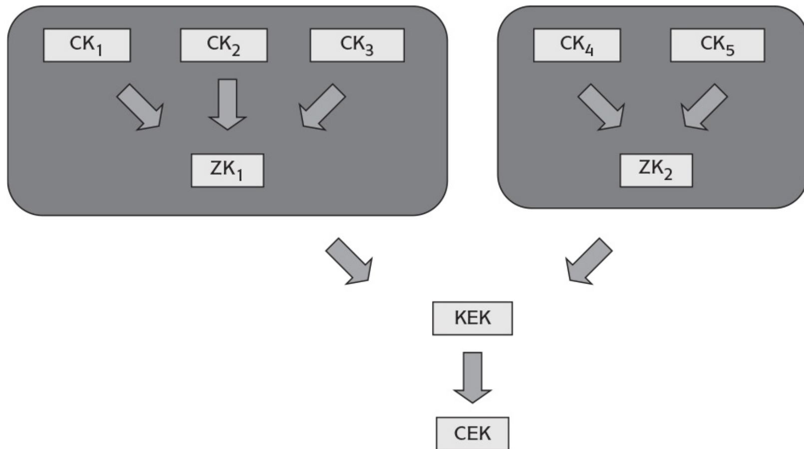
Figure 12.12: Digital video broadcast scheme key hierarchy.
