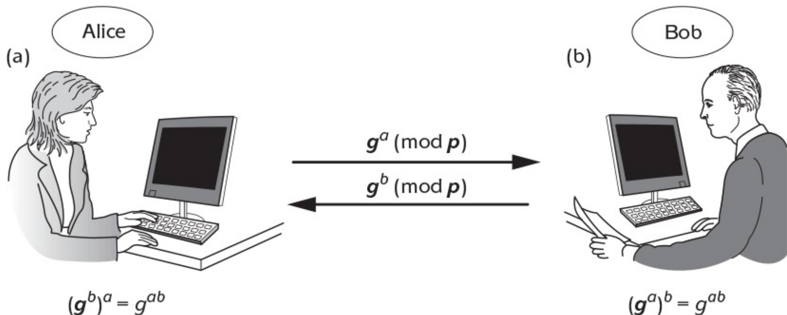
Figure 9.10: Diffie–Hellman protocol.
