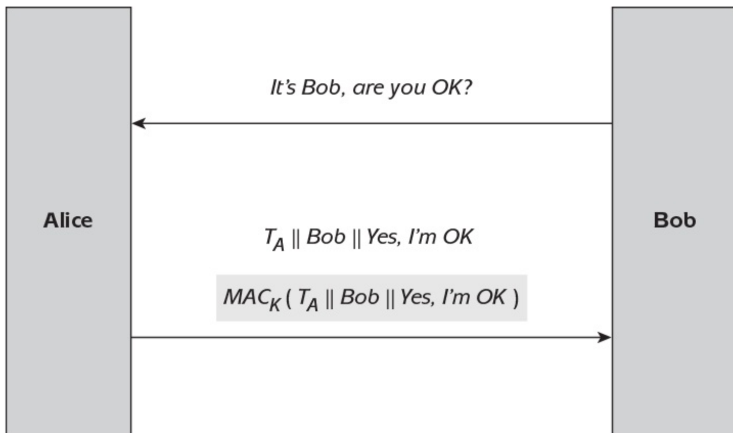
Figure 9.8: Protocol 6.
