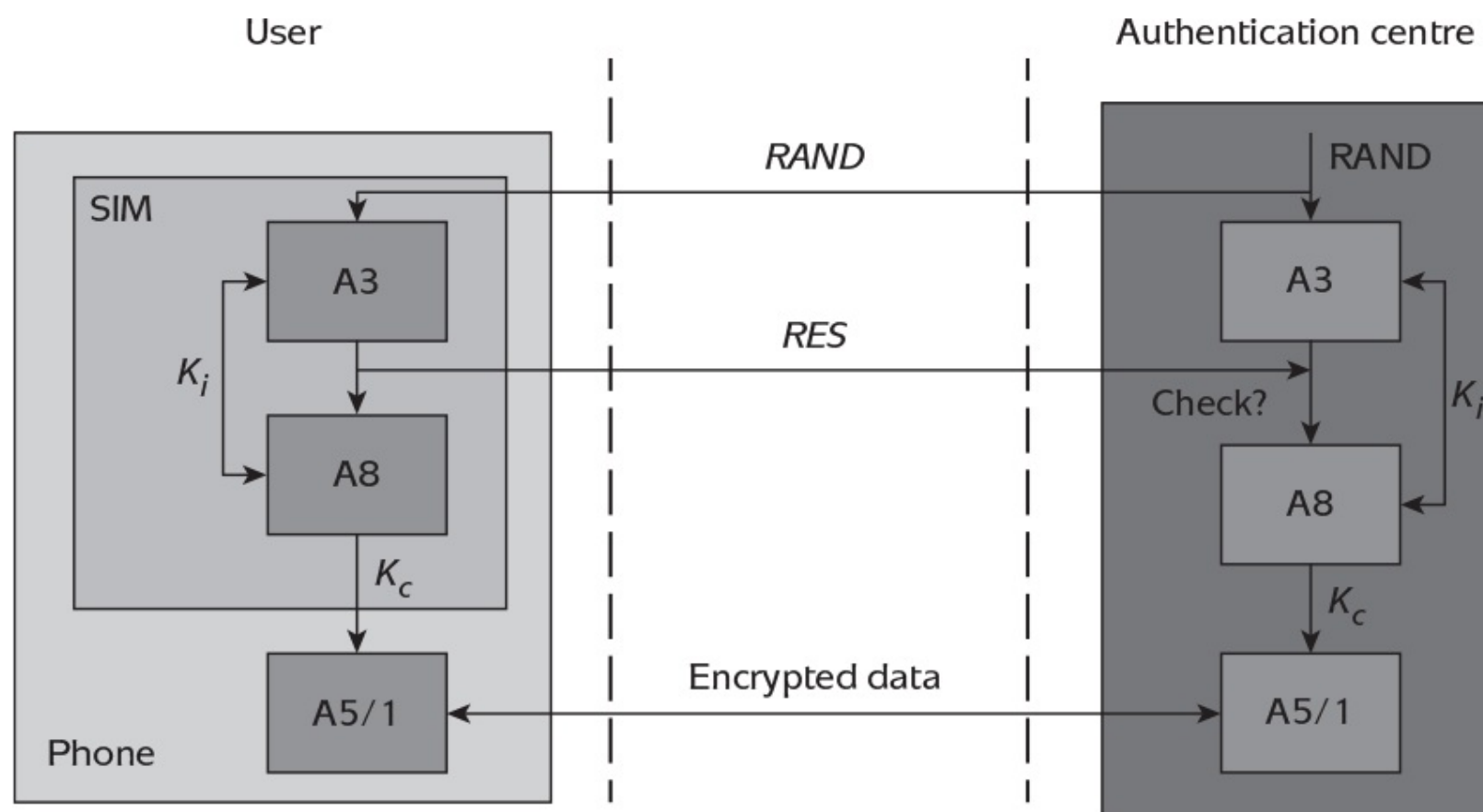
Figure 12.8: GSM authentication and encryption.
