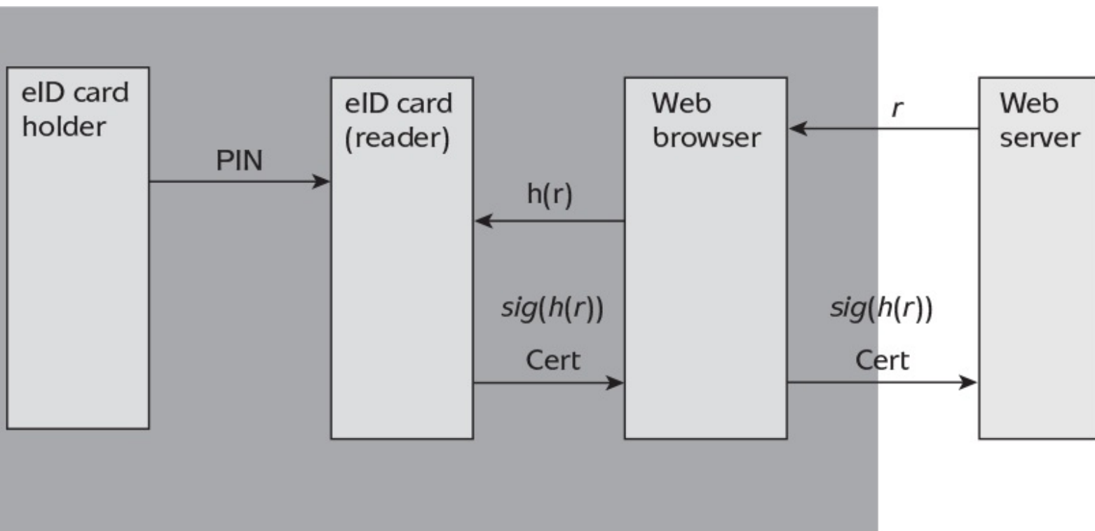
Figure 12.14: eID card holder authentication.
