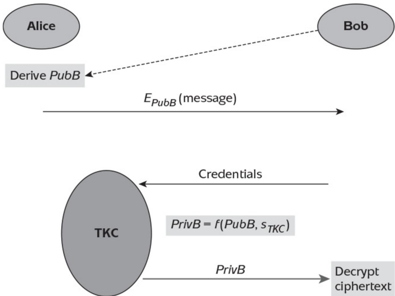
Figure 11.8: The IBE process.
