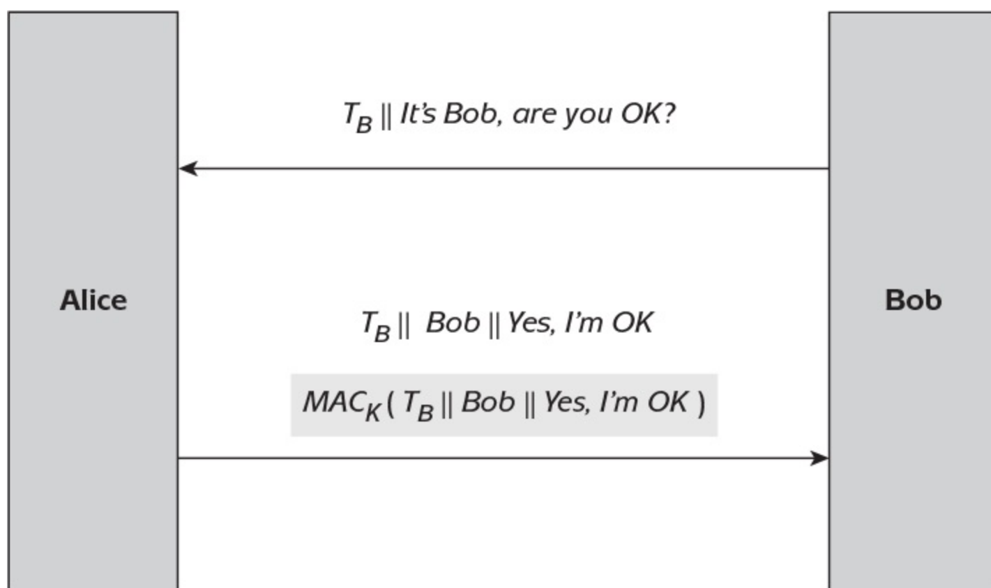
Figure 9.7: Protocol 5.
