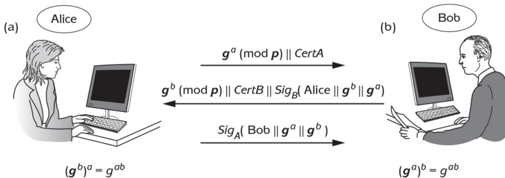
Figure 9.12: Station-to-station protocol.
