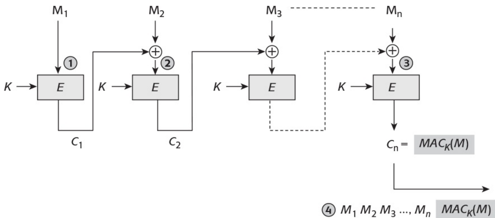
Figure 6.8: CBC-MAC.
