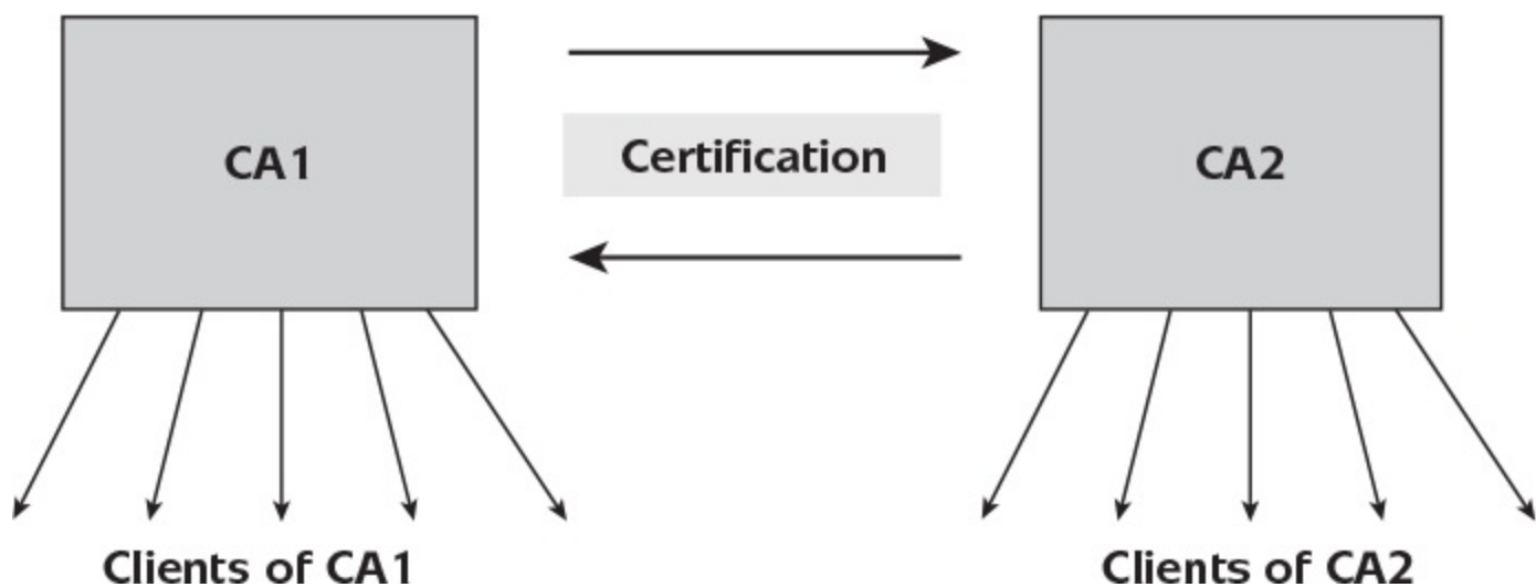
Figure 11.5: Cross-certification.
