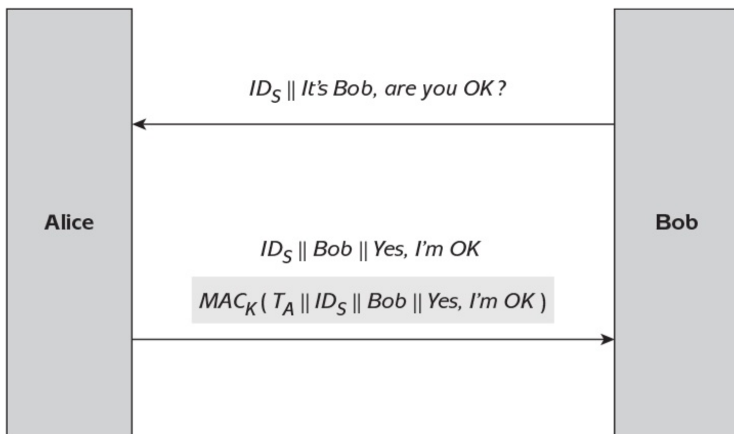
Figure 9.9: Protocol 7.
