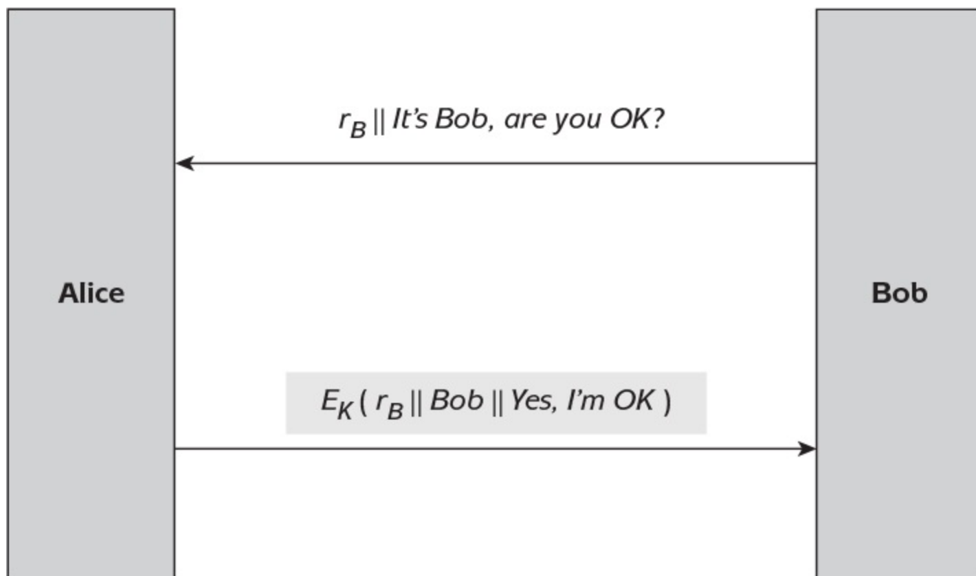
Figure 9.6: Protocol 4.
