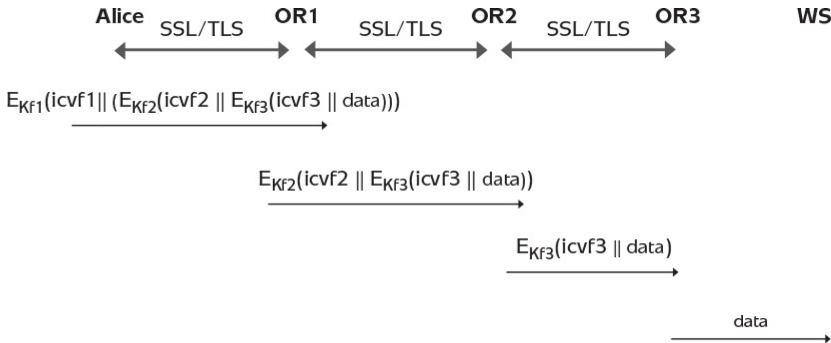
Figure 12.18: Tor communication.
