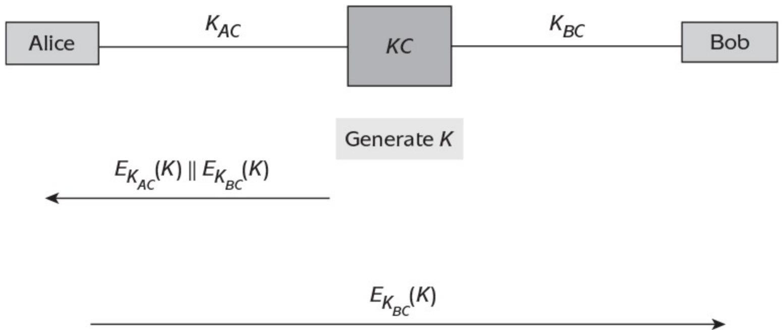
Figure 10.4: Key despatch.
