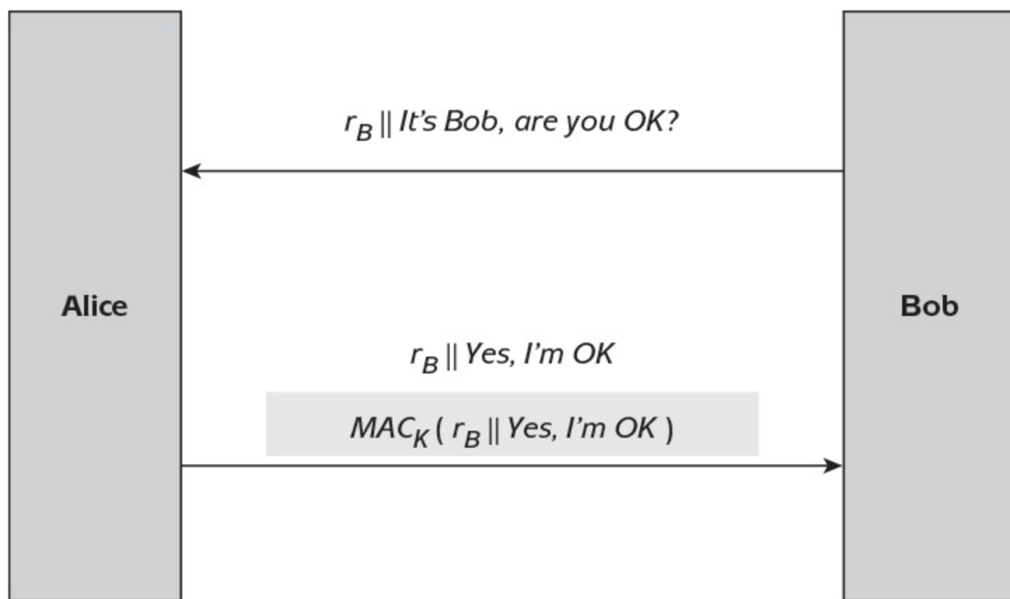
Figure 9.4: Protocol 3.
