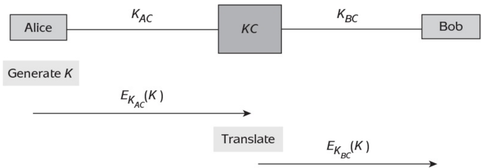
Figure 10.3: Key translation.
