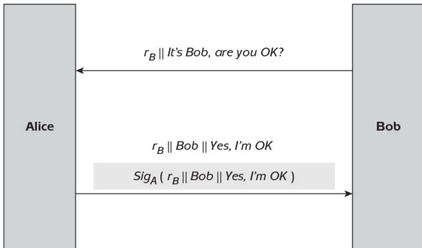
Figure 9.3: Protocol 2.
