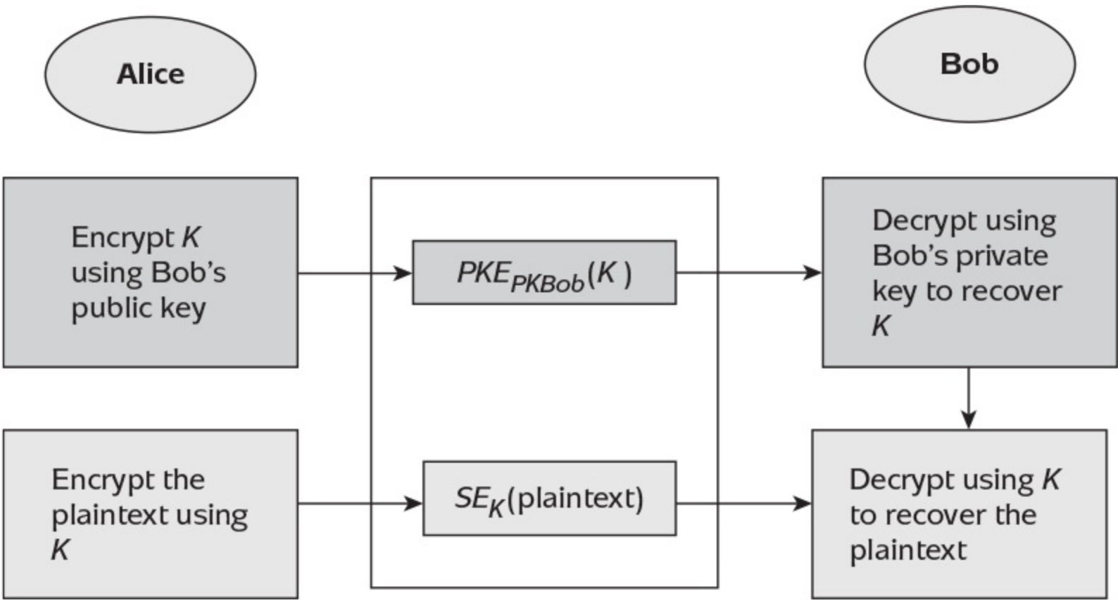
Figure 5.2: Hybrid encryption.
