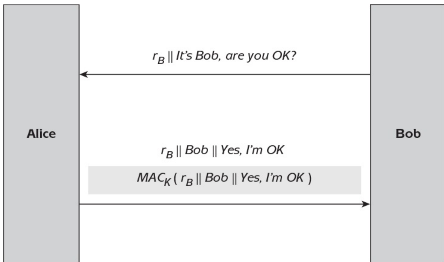
Figure 9.2: Protocol 1.
