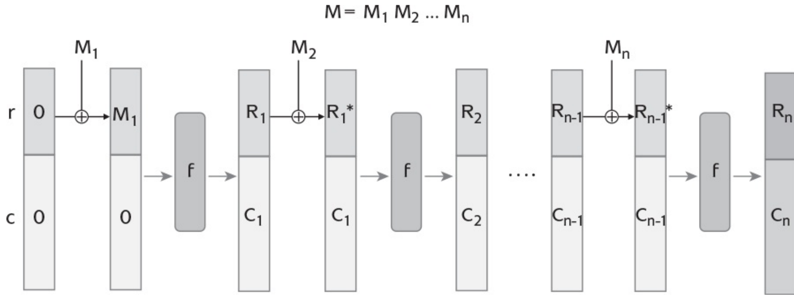
Figure 6.6: Hash function sponge construction for SHA-3.
