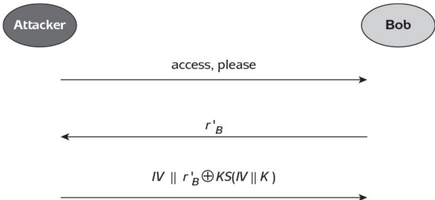
Figure 12.5: Keystream replay attack on WEP authentication.
