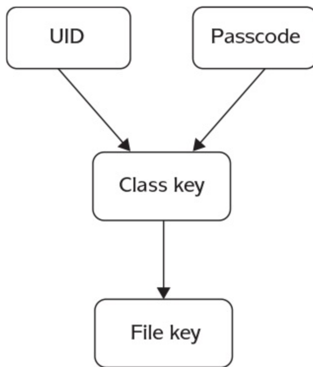
Figure 13.2: iOS key hierarchy.
