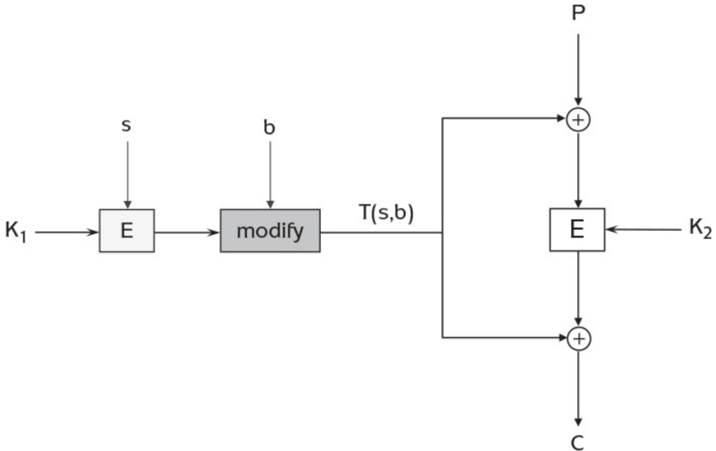
Figure 13.1: Encryption using XTS mode.
