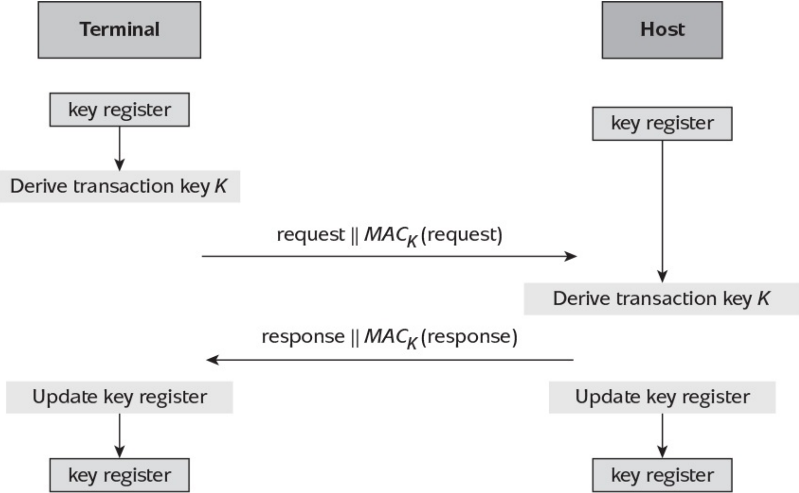
Figure 10.5: Generic UKPT scheme.
