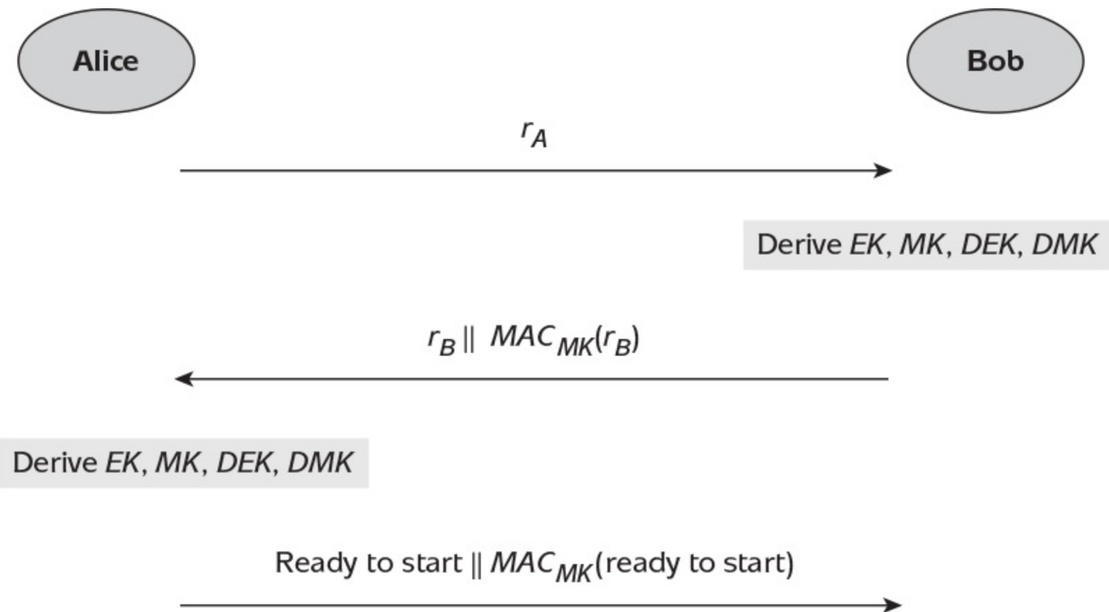
Figure 12.6: WPA authentication and key establishment protocol.
