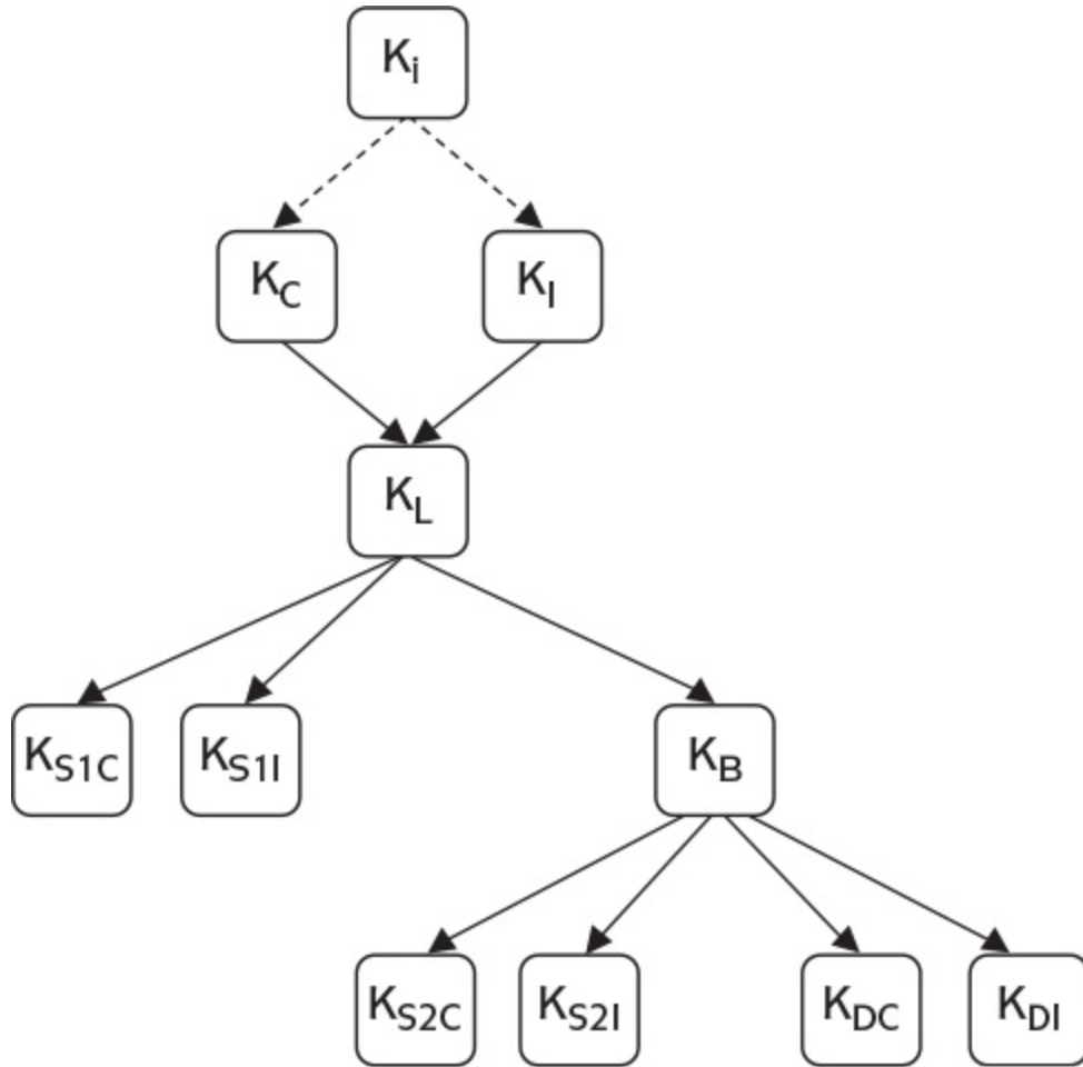
Figure 12.9: LTE key hierarchy.
