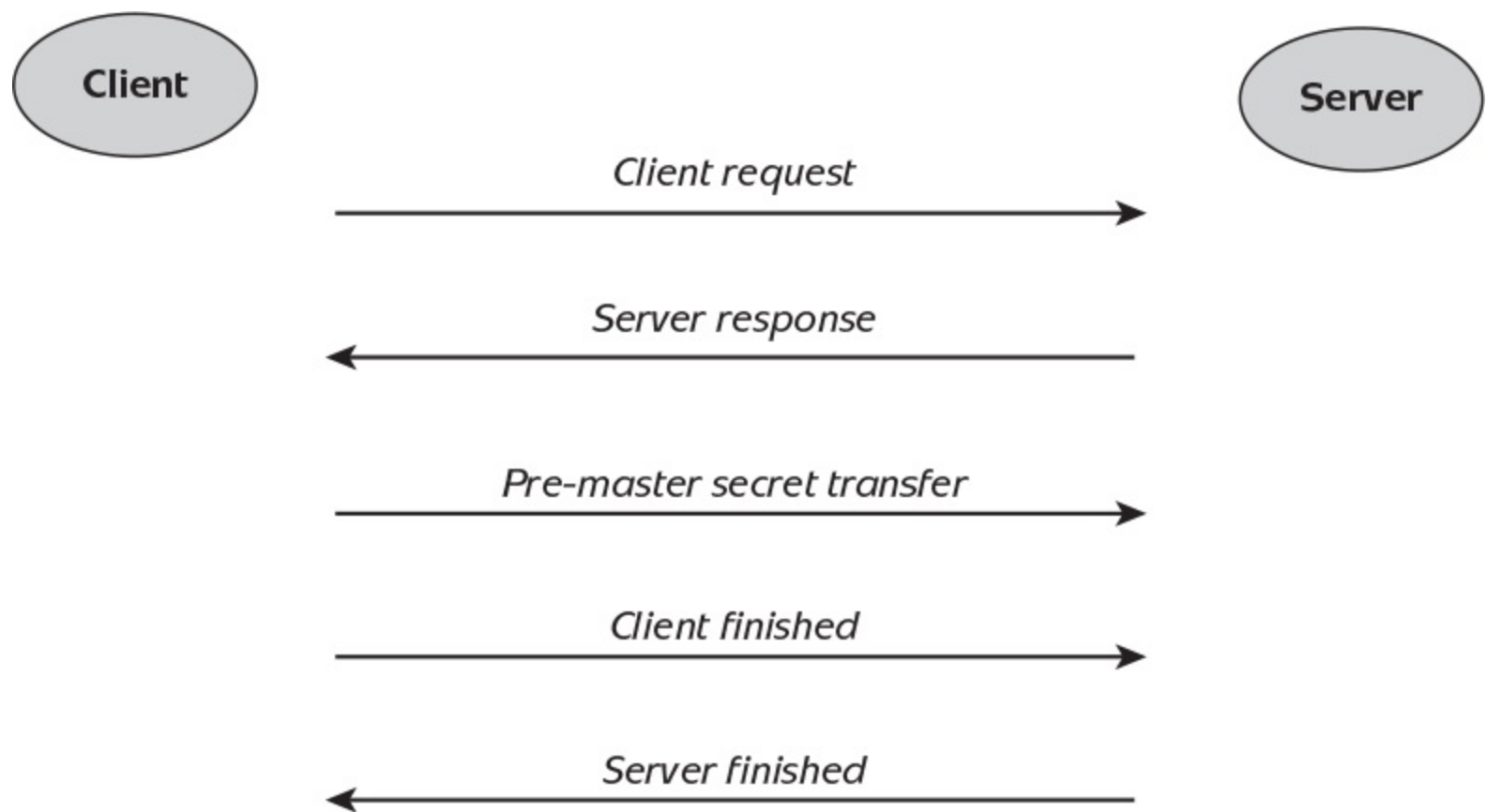
Figure 12.1: Handshake Protocol for TLS 1.2 and earlier versions.
