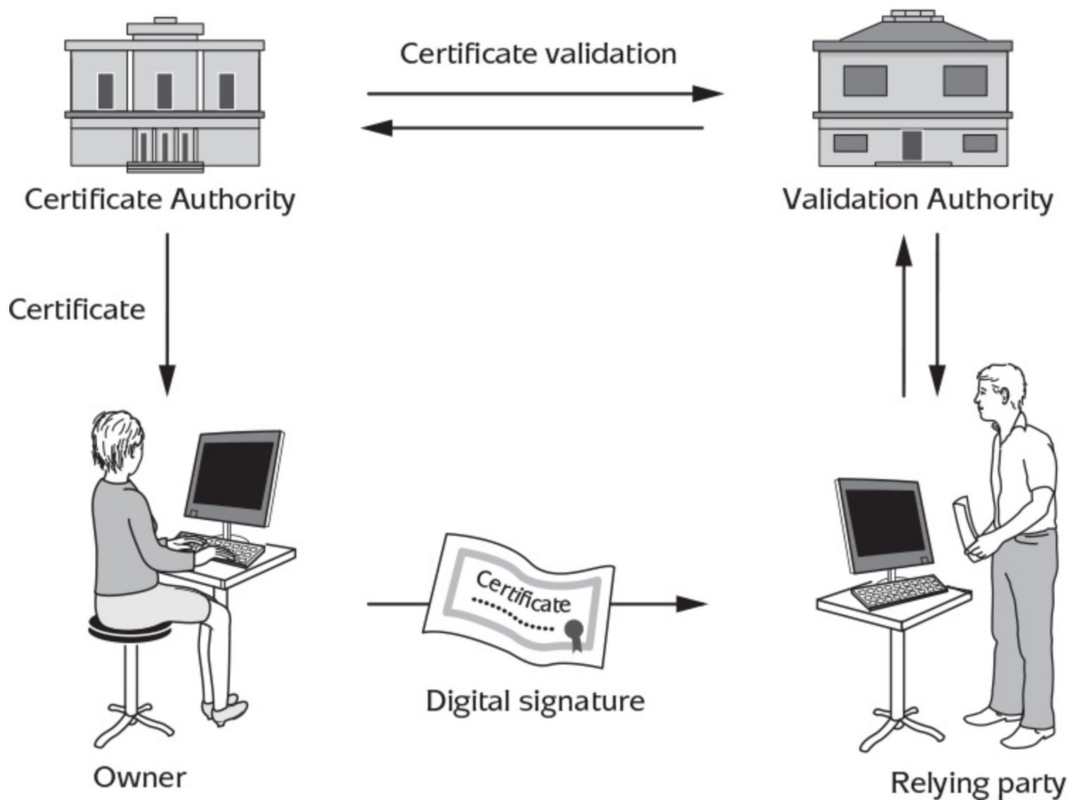
Figure 11.4: Connected certification model.
