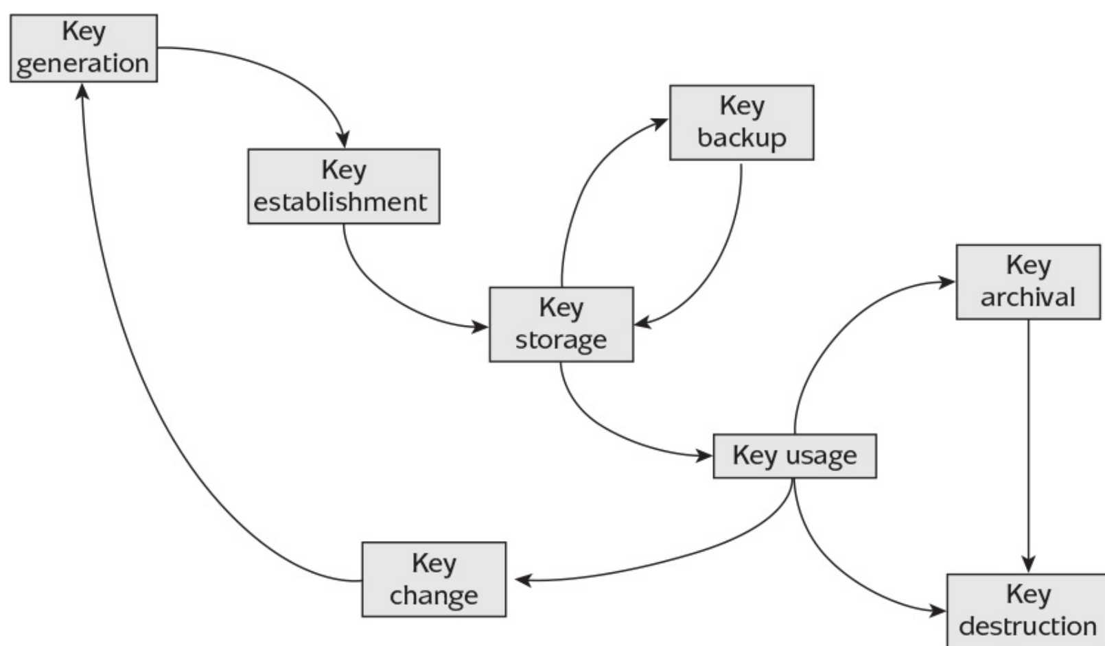
Figure 10.1: The key lifecycle.
