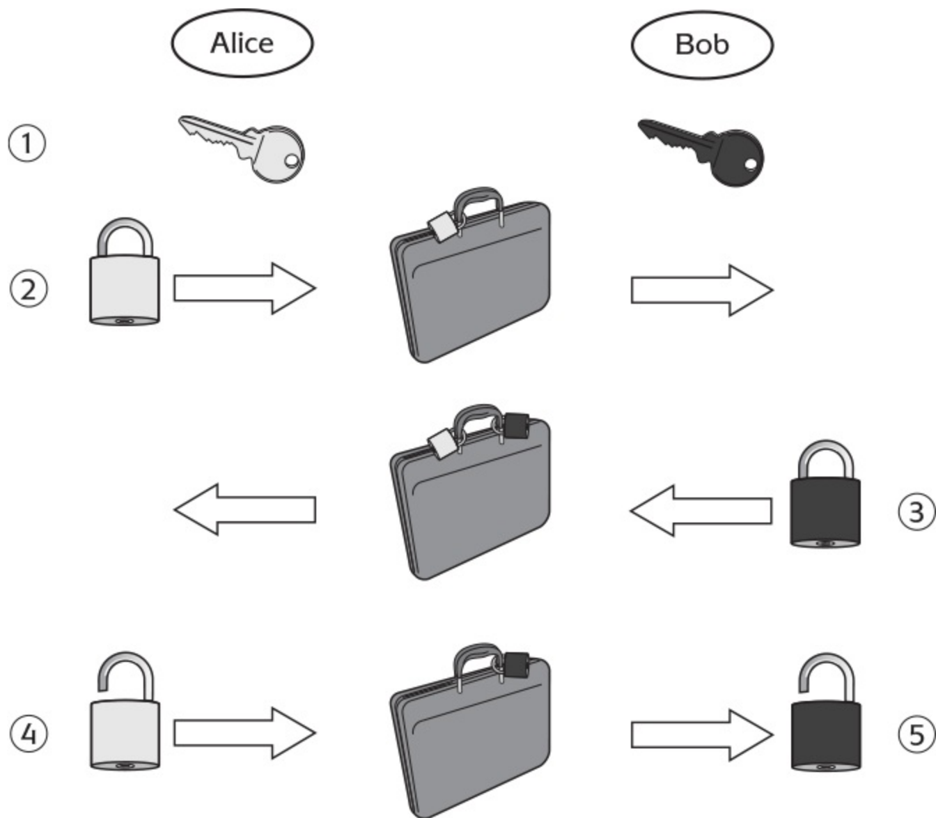
Figure 5.1: The briefcase protocol.
