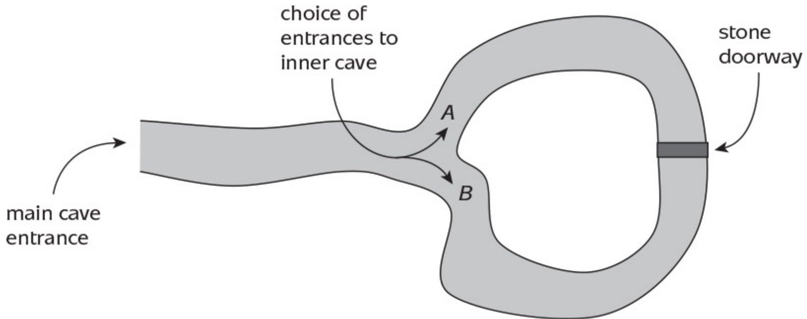
Figure 8.4: Popular analogy of a zero-knowledge mechanism.
