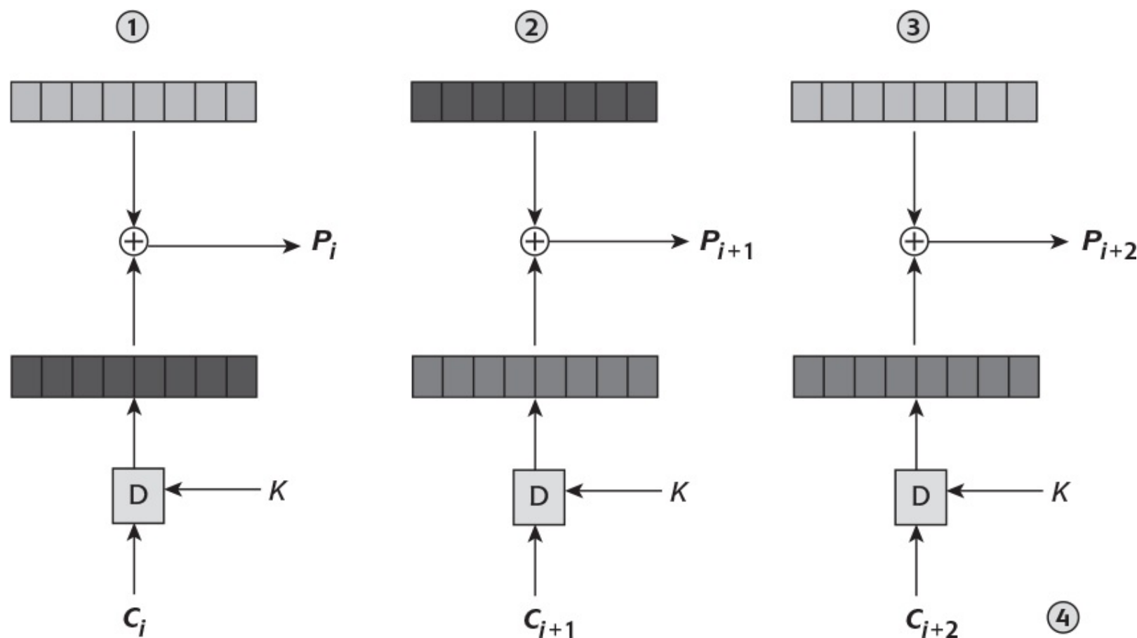
Figure 4.11: Effect of a 1-bit transmission error using CBC mode.
