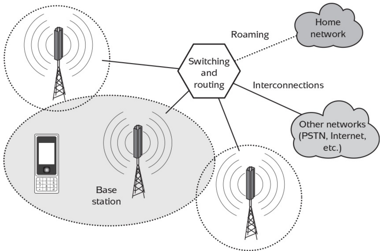
Figure 12.7: Basic architecture of mobile telecommunications network.
