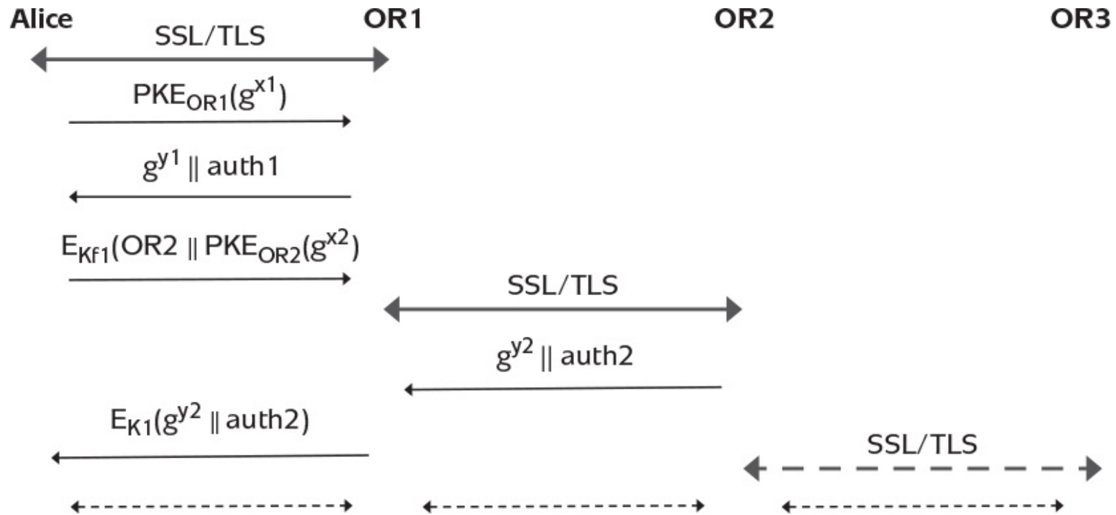
Figure 12.17: Tor key establishment.
