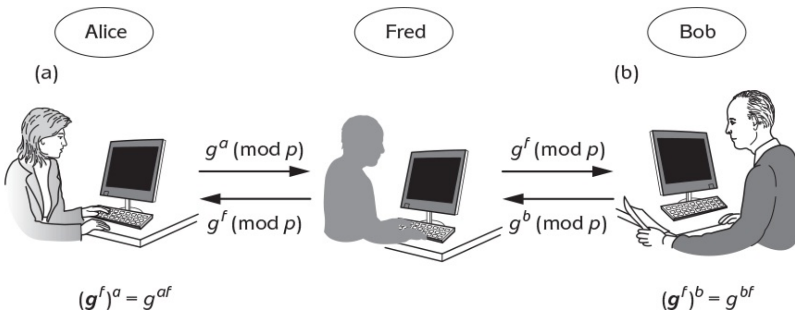
Figure 9.11: Man-in-the-middle attack against the Diffie–Hellman protocol.
