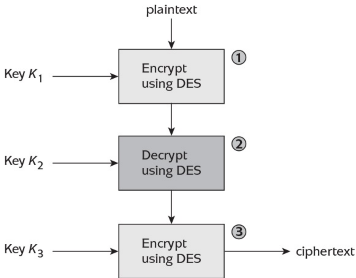
Figure 4.6: Encryption using 3TDES.
