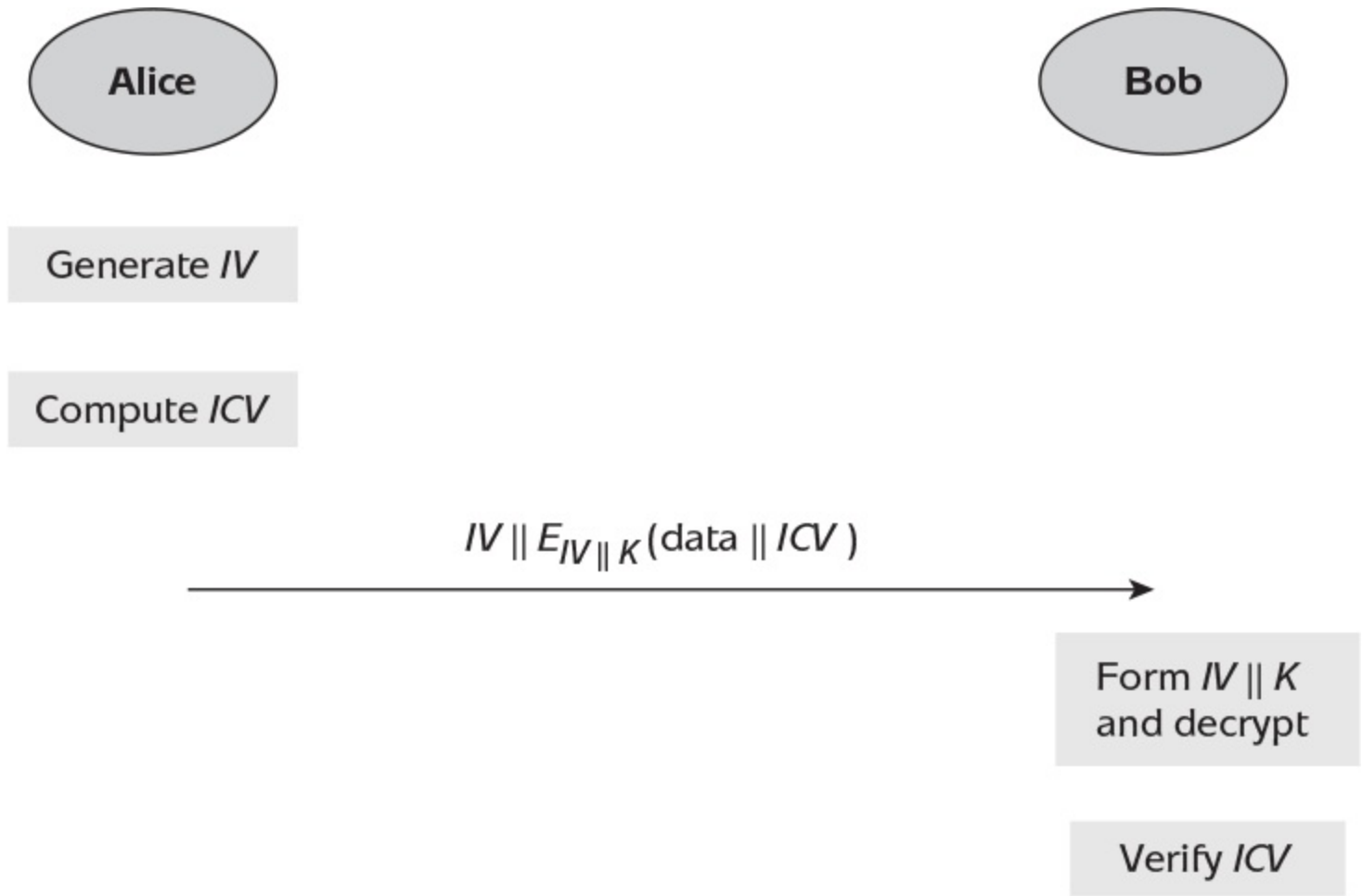
Figure 12.4: WEP encryption process.
