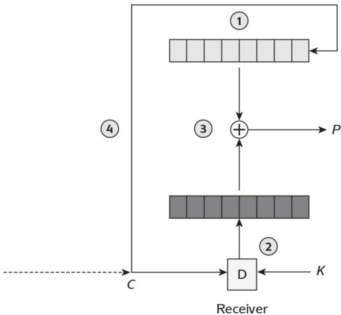
Figure 4.10: Decryption using CBC mode.
