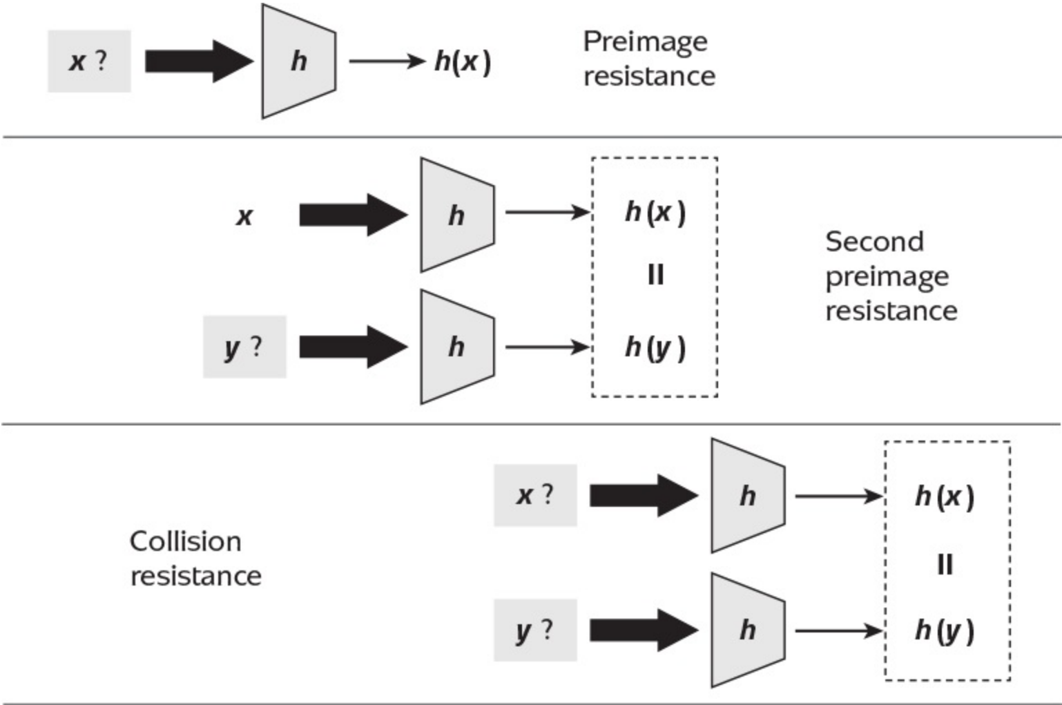
Figure 6.1: Three security properties of a hash function.
