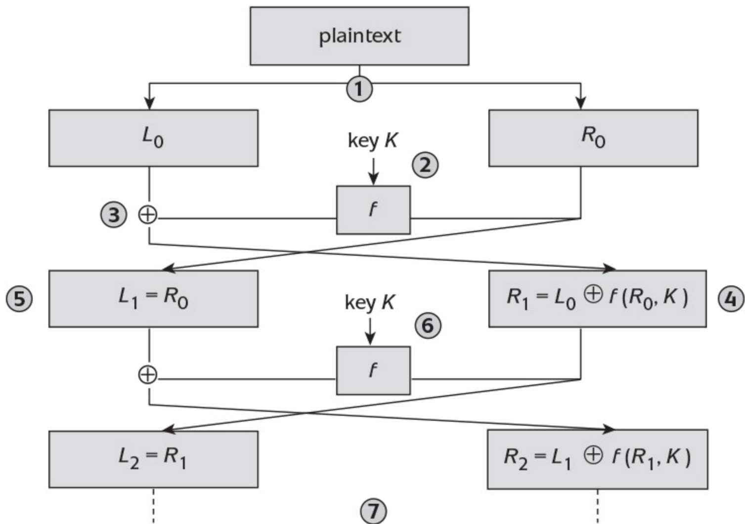
Figure 4.5: A Feistel Cipher.
