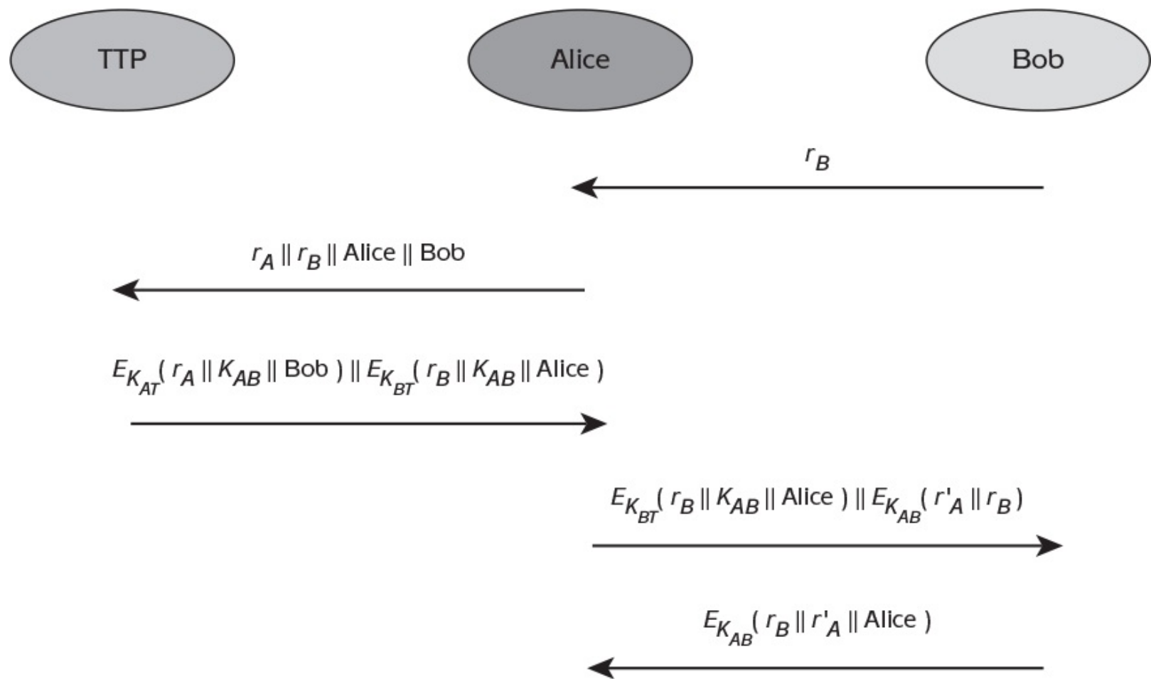
Figure 9.13: An AKE protocol from ISO 9798-2.
