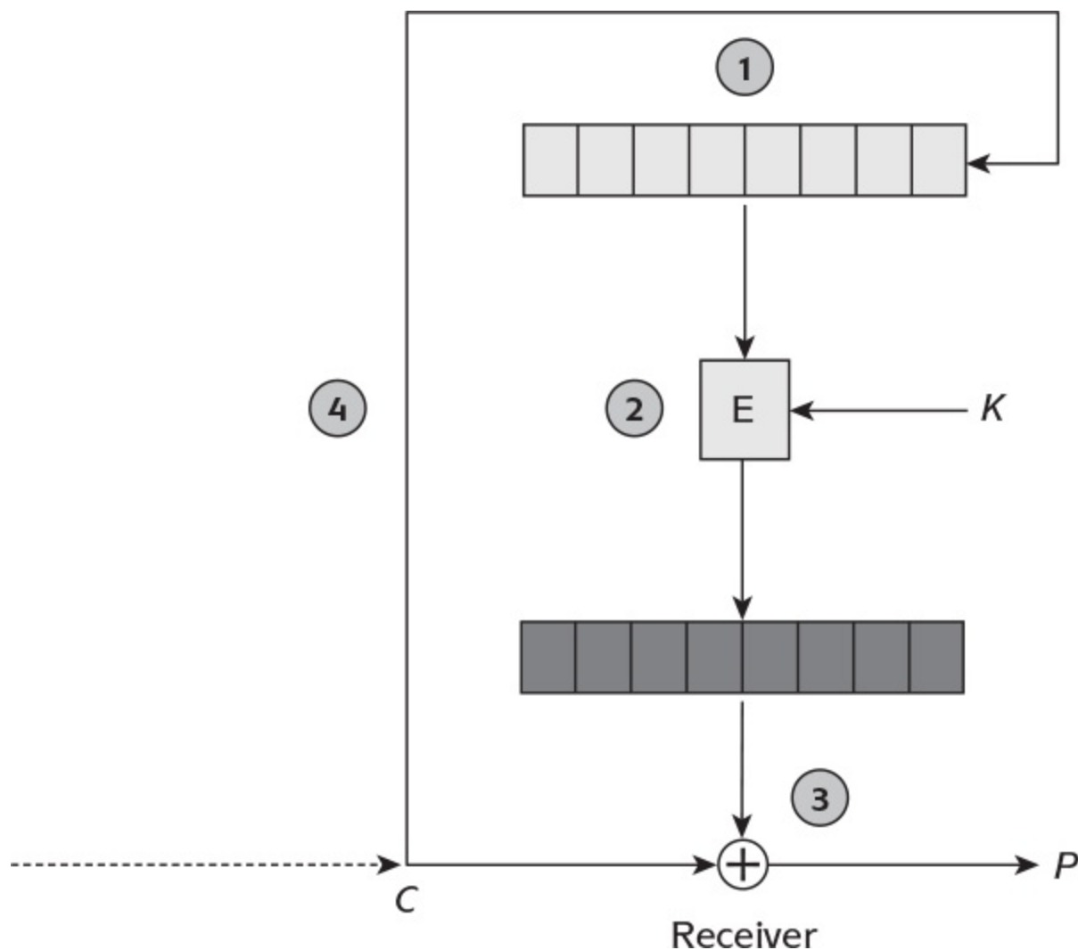
Figure 4.13: Decryption using CFB mode.
