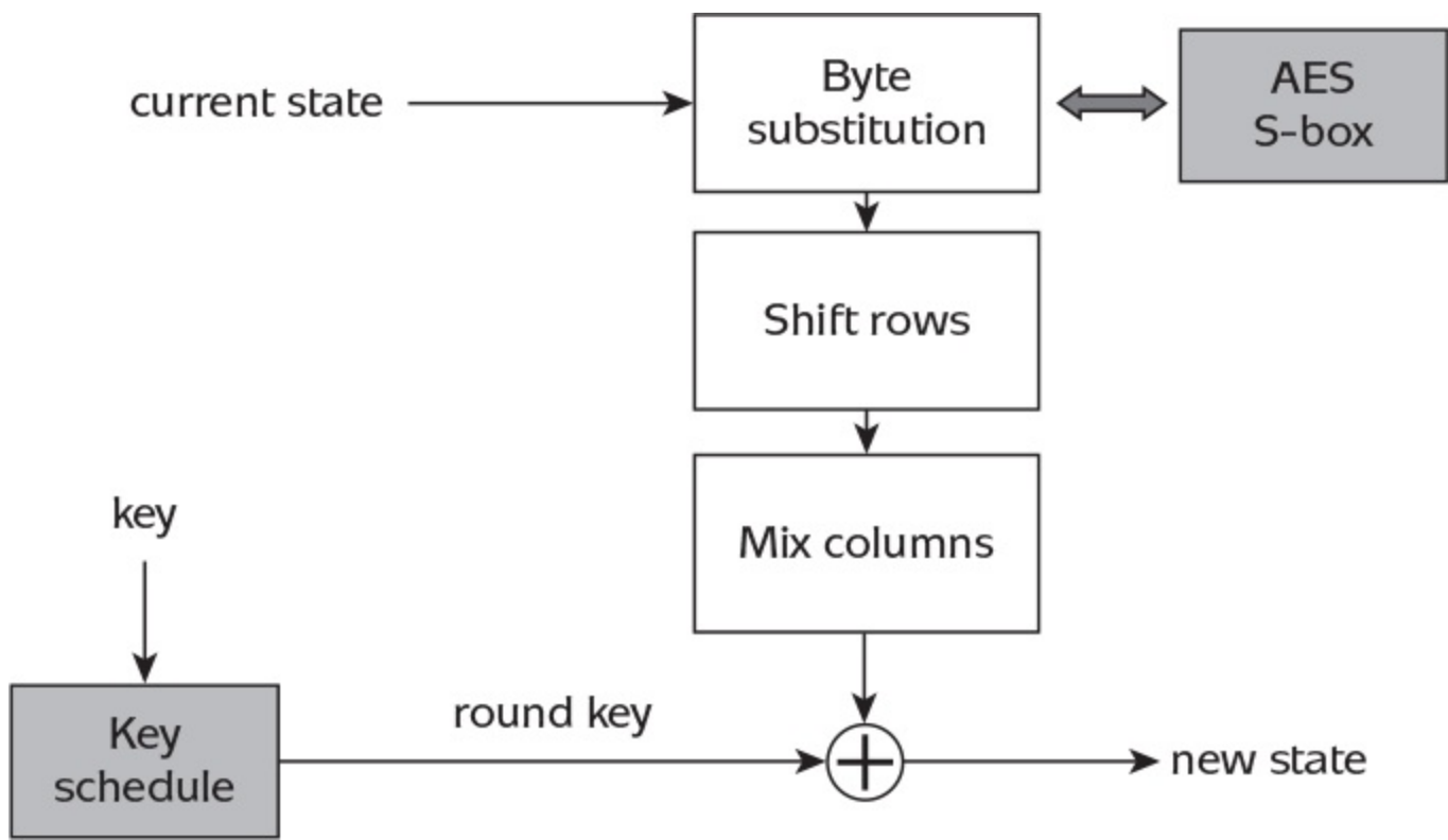
Figure 4.7: One AES encryption round.
