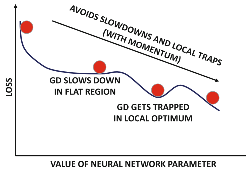
Figure 3.12: Effect of momentum in navigating complex loss surfaces. The annotation “GD” indicates pure gradient descent without momentum. Momentum helps the optimization process retain speed in flat regions of the loss surface and avoid local optima.
