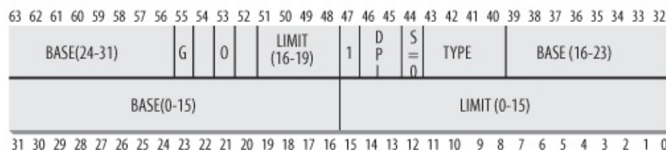
Figure 2-3. Segment Descriptor format
