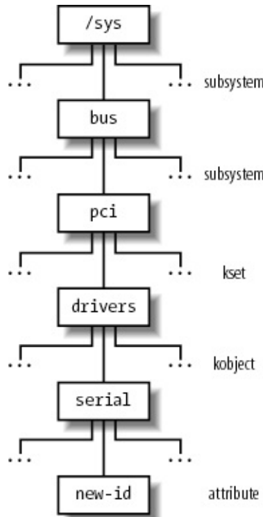
Figure 13-3. An example of device driver model hierarchy
