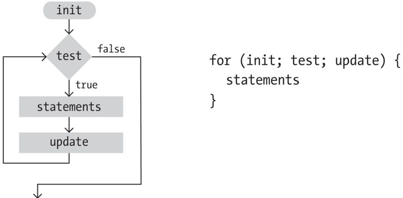
Figure 4-1. Flow diagram of a for loop
