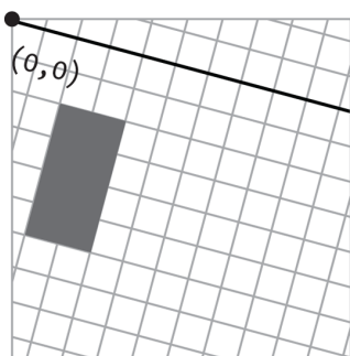
Figure 6-2. Rotating the coordinates
