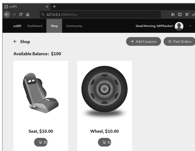
Figure 5-1: The crAPI shop
