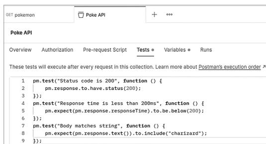
Figure 4-27: Poke API tests
