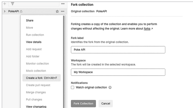
Figure 4-20: Forking an API collection in Postman
