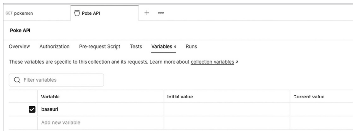
Figure 4-23: The Poke API collection variables
