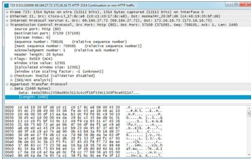
FIGURE 5.1 Sample PCAP Data as seen in Wireshark
