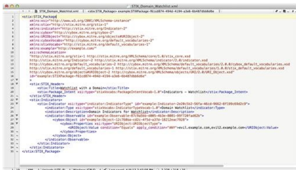
FIGURE 7.10 A STIX Indicator with Domains in a Watch list
