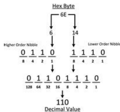
FIGURE 13.7 Converting Hexadecimal to Binary and Decimal
