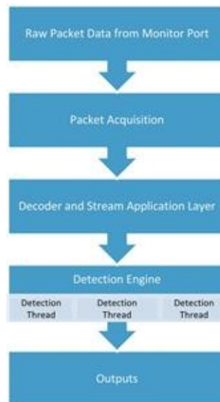
FIGURE 9.7 The Default Suricata Runmode
