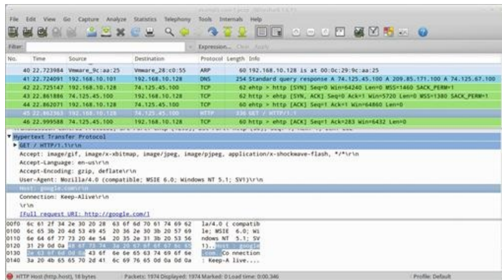
FIGURE 13.30 Viewing Packets in Wireshark
