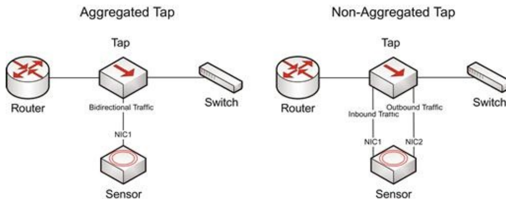
FIGURE 3.7 Aggregated and Non-Aggregated Taps
