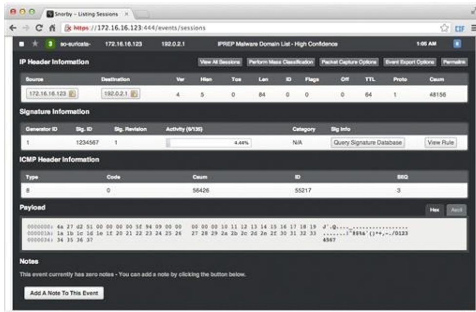
FIGURE 8.13 An Alert Generated by the Suricata Iprep Directive
