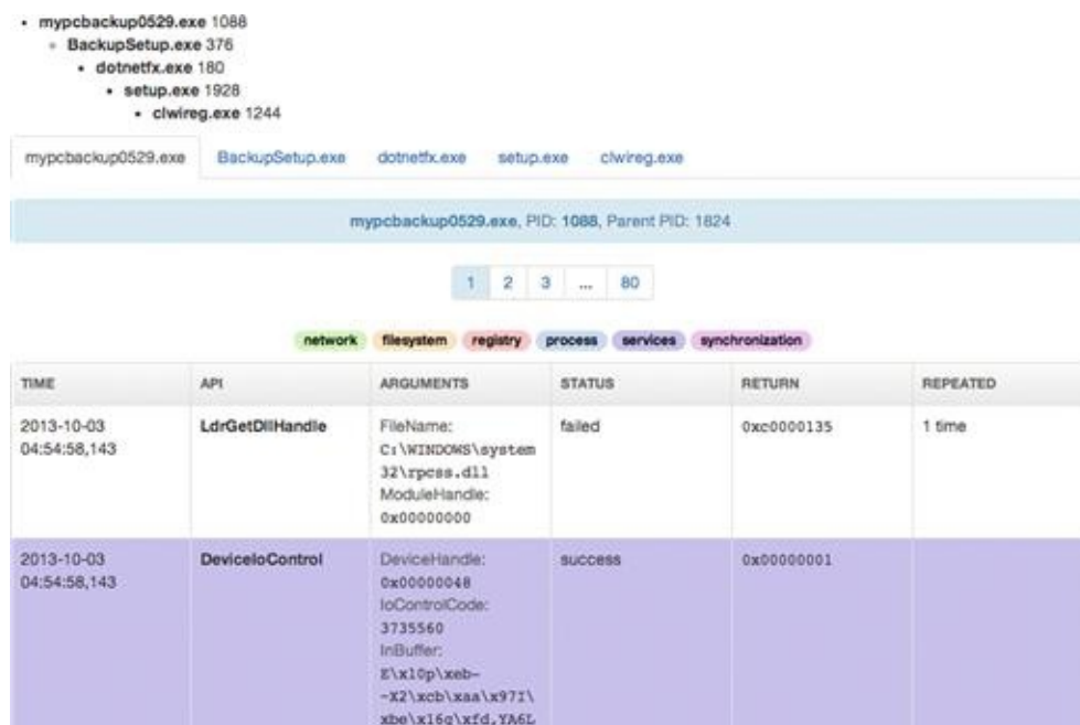
FIGURE 14.21 Cuckoo Report Showing Behavioral Analysis Results
