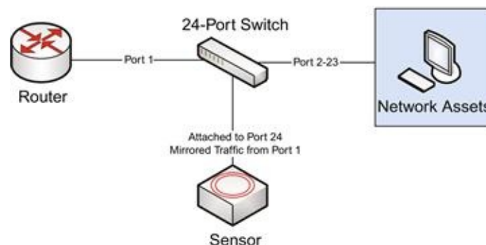
FIGURE 3.5 Using a SPAN Port to Capture Packets
