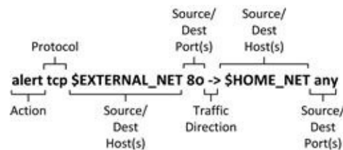
FIGURE 9.20 The IDS Rule Header
