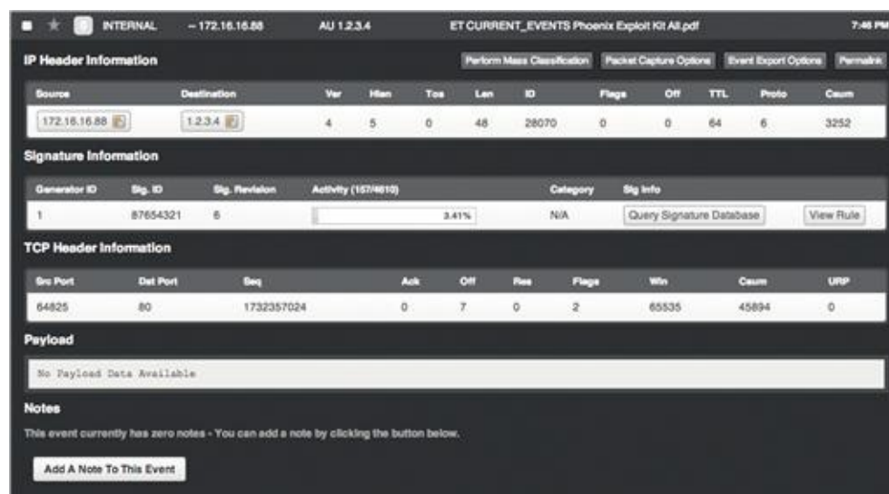
FIGURE 3.15 A User in Scenario B Generating an Alert
