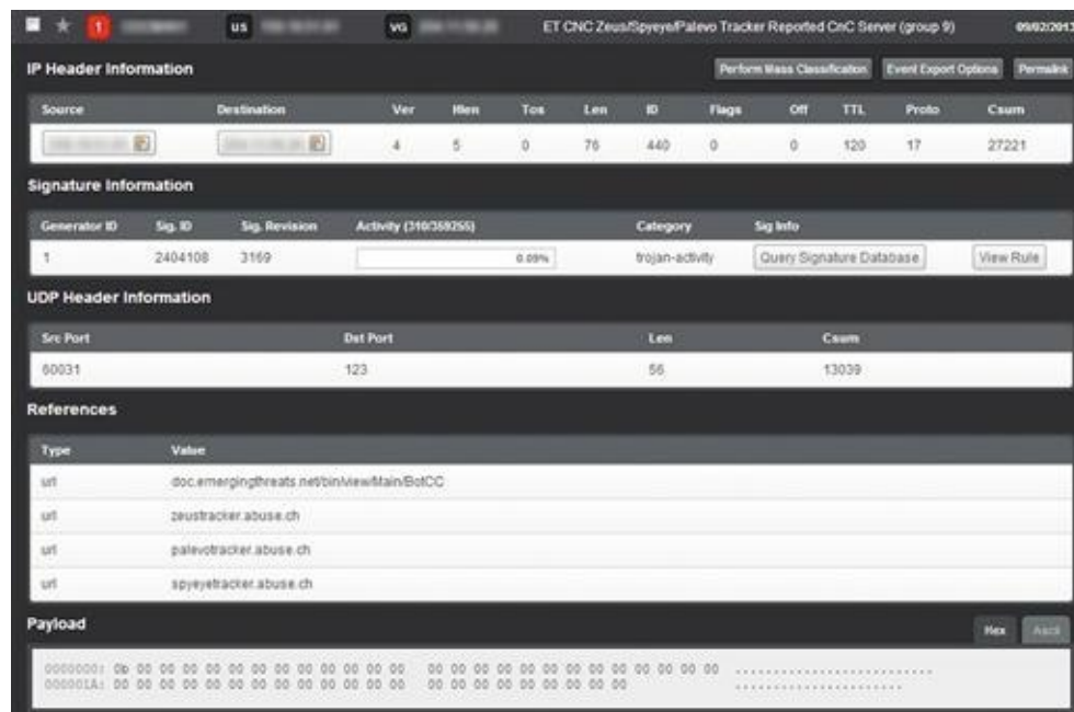
FIGURE 11.7 A Zeus Alert Generated by Snort
