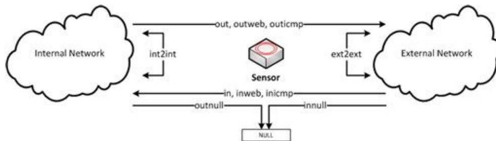
FIGURE 4.5 SiLK Flow Types
