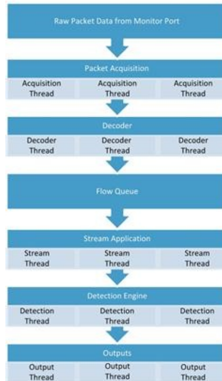
FIGURE 9.8 The Pfring Suricata Runmode
