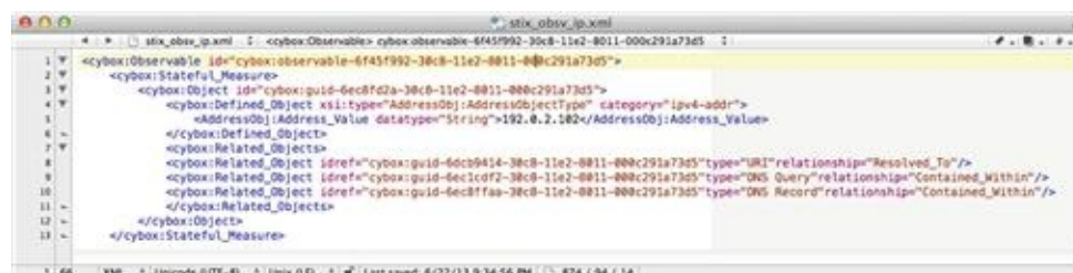
FIGURE 7.9 A STIX Observable Representing an IP Address with Related Objects
