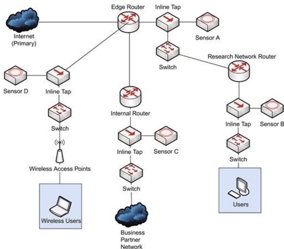
FIGURE 3.11 Placing Sensors at Network Ingress/Egress Points
