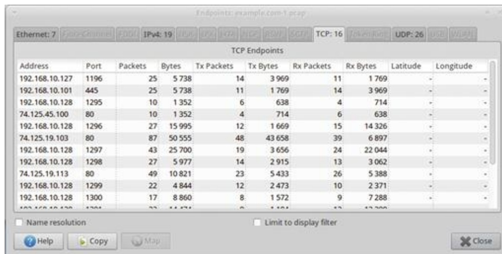
FIGURE 13.33 Wireshark's Endpoints Window
