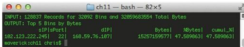
FIGURE 11.3 Using Statistics to Identify Service Usage
