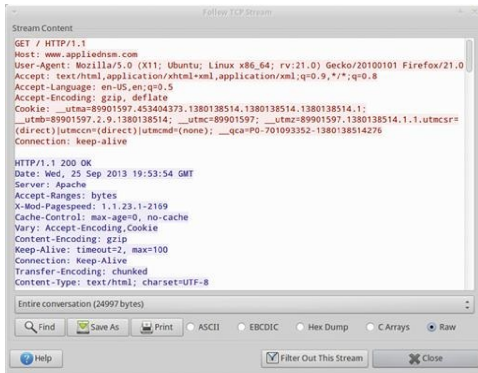
FIGURE 13.35 Following a TCP Stream
