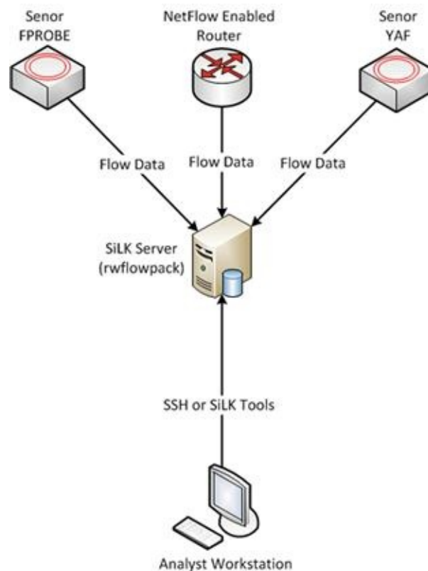
FIGURE 4.4 The SiLK Workflow
