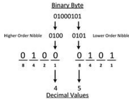
FIGURE 13.4 Calculating the Decimal Value of Each Nibble
