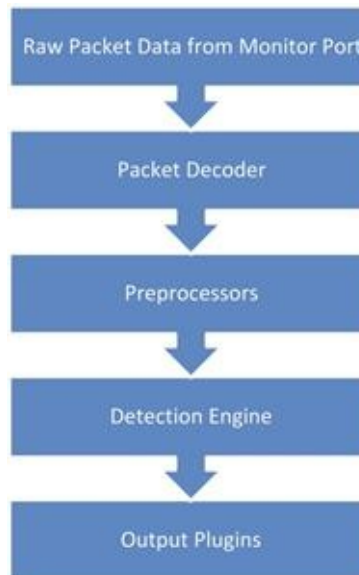
FIGURE 9.4 The Snort NIDS Mode Architecture
