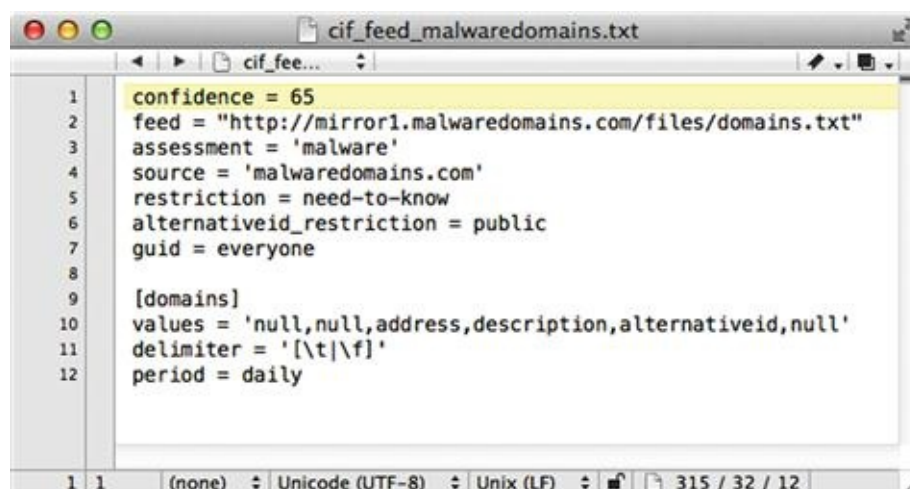
FIGURE 8.7 A CIF Feed Configuration File for a Delimited Text List
