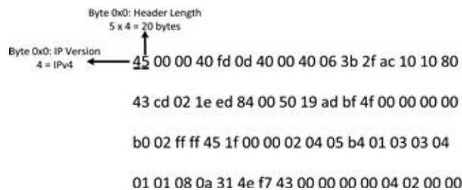
FIGURE 13.11 The IP Version and Header Length Fields at 0 × 0
