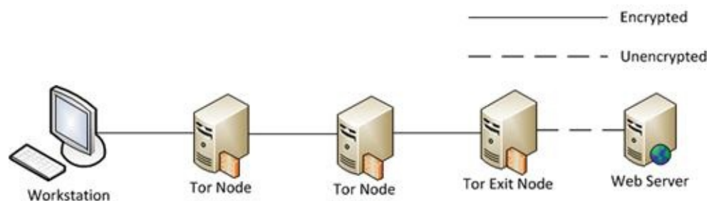
FIGURE 8.2 Tor Communication Process
