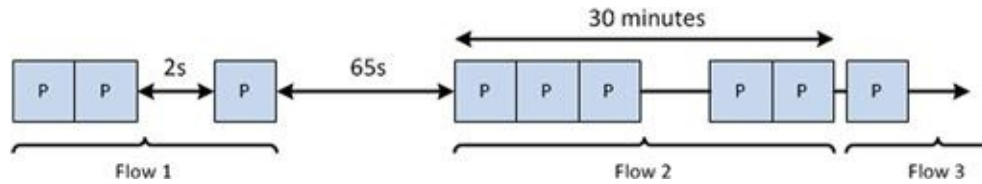
FIGURE 4.2 Flow Idle and Active Termination
