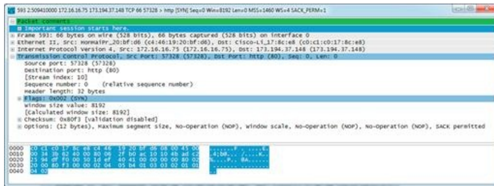
FIGURE 5.2 A Commented Packet Leveraging PCAP-NG
