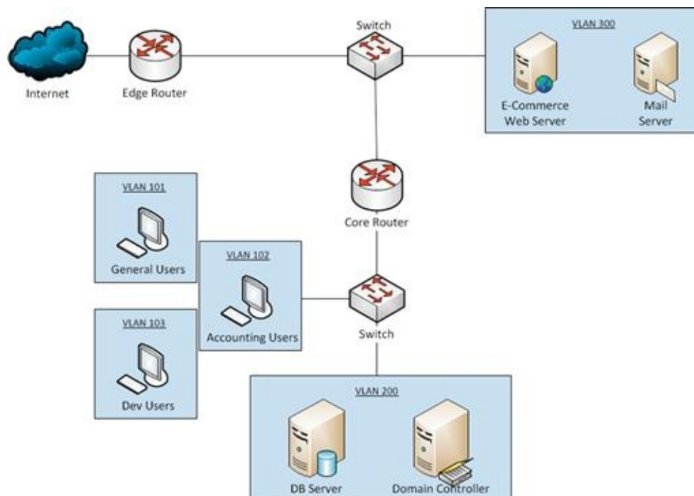
FIGURE 2.2 Purple Dog Inc. Network Diagram
