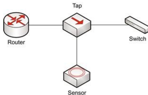
FIGURE 3.6 Using a Network Tap to Capture Packets
