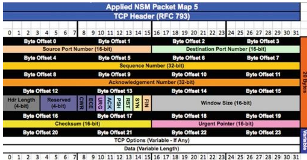
FIGURE 13.16 Packet Map for the TCP Header
