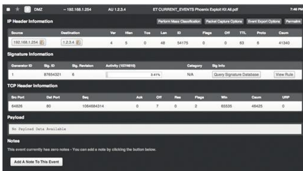
FIGURE 3.13 A User in Scenario A Generating an Alert
