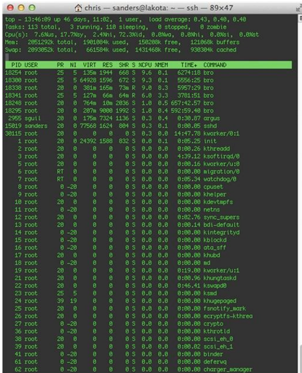
FIGURE 3.3 Monitoring Sensor CPU Usage with TOP
