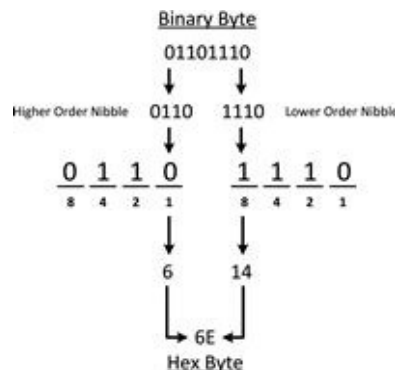
FIGURE 13.6 Converting Another Binary Byte to Hex
