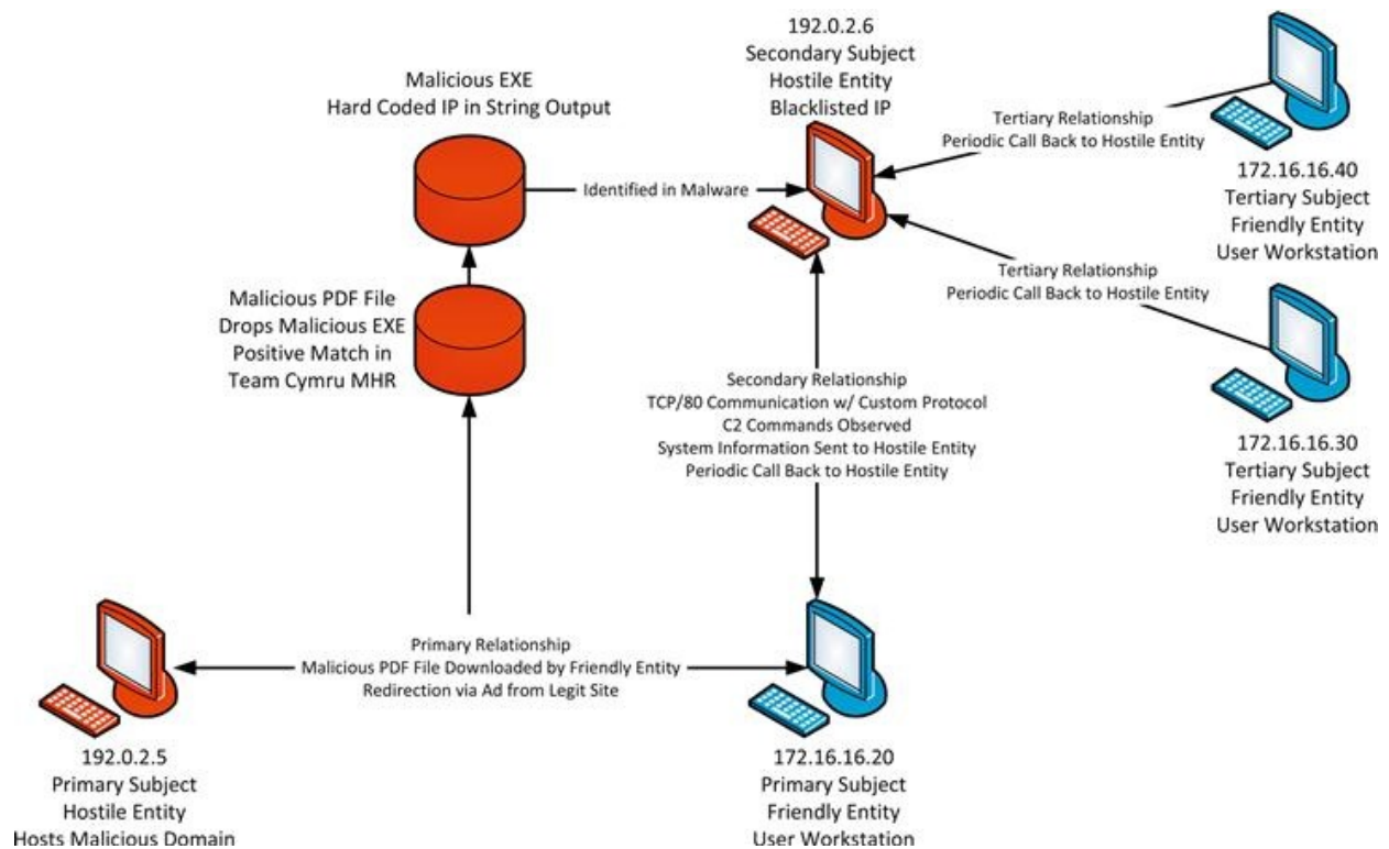
FIGURE 15.5 Relationship of All Subjects
