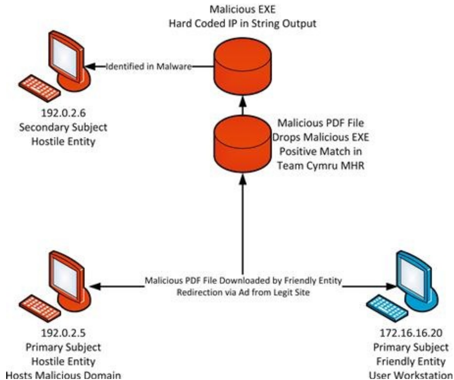
FIGURE 15.3 Relationship of Primary Subjects
