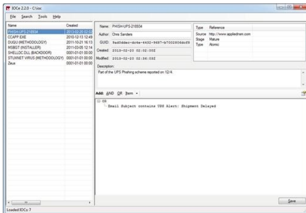
FIGURE 7.7 Mandiant's OpenIOC Editor for Windows
