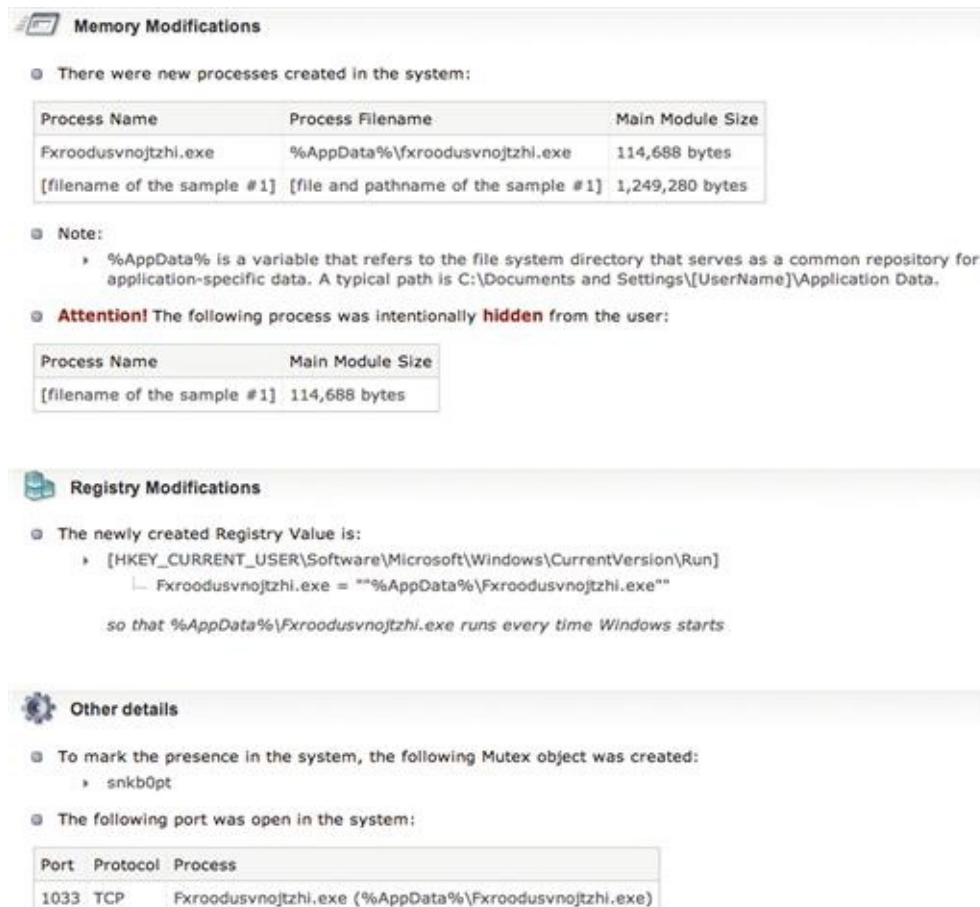
FIGURE 14.23 ThreatExpert Report Detailing Multiple Actions
