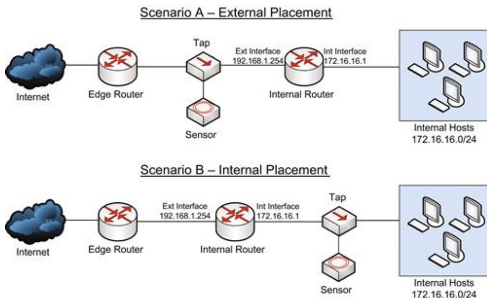
FIGURE 3.12 A Simple Network with Two Sensor Placement Examples
