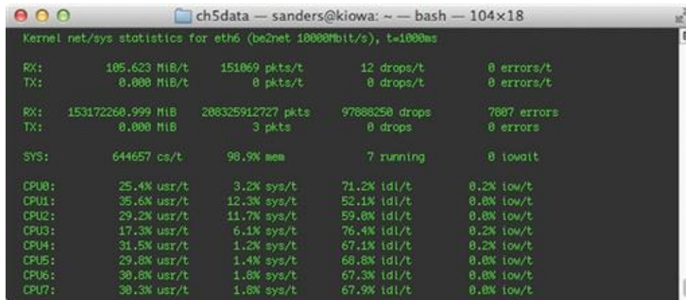
FIGURE 5.4 Generating Network Statistics with ifpps
