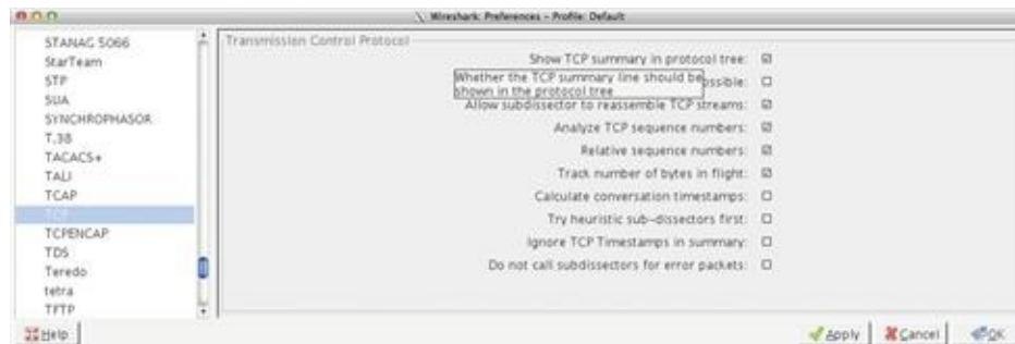
FIGURE 13.39 Protocol Dissector Options for the TCP Protocol
