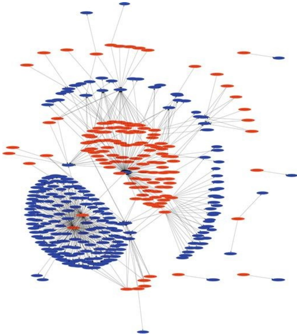
FIGURE 11.13 A Link Graph Created from NetFlow Data
