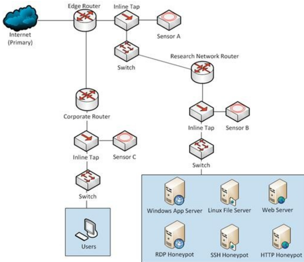
FIGURE 12.1 Canary Honeypot Placement Near Protected Assets
