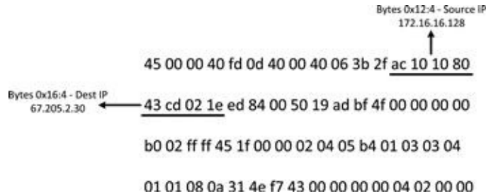
FIGURE 13.12 The Source and Destination IP Address Fields at 0x12 and 0x16
