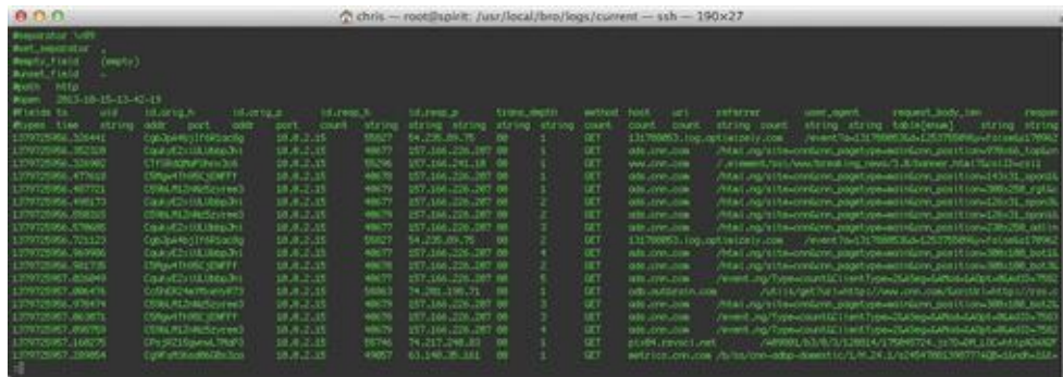
FIGURE 10.2 Partial http.log file contents
