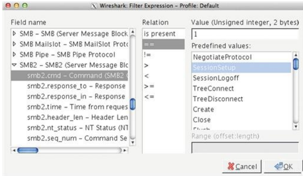
FIGURE 13.41 Building Display Filters with the Expression Builder
