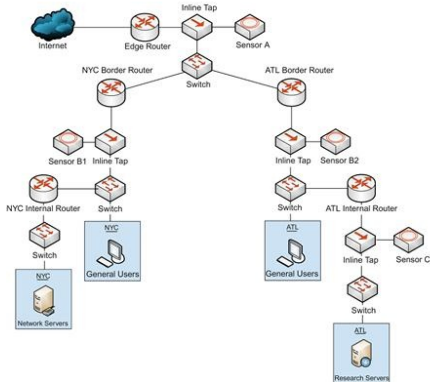
FIGURE 3.17 A Mid-Sized Network with Three Sensor Placement Examples
