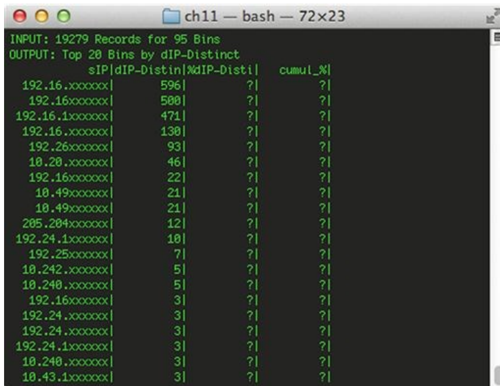
FIGURE 11.9 Showing Multiple Devices Exhibiting Similar Communication Patterns
