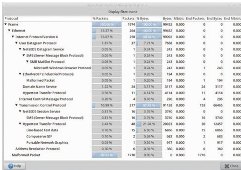
FIGURE 13.32 Wireshark's Protocol Hierarchy Window
