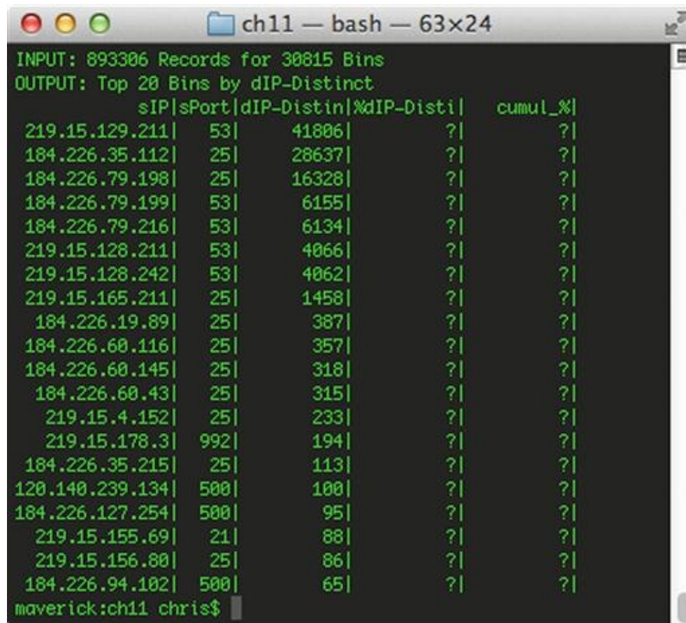
FIGURE 11.5 Top Communicating Server Ports
