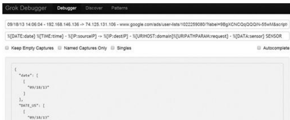
FIGURE 6.15 Using the Grok Debugger
