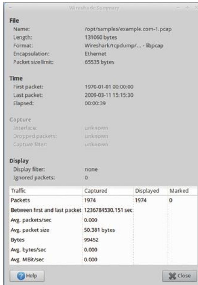
FIGURE 13.31 Wireshark's Summary Window
