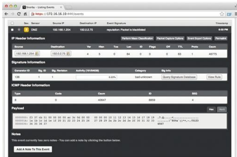
FIGURE 8.12 An Alert Generated by the Reputation Preprocessor
