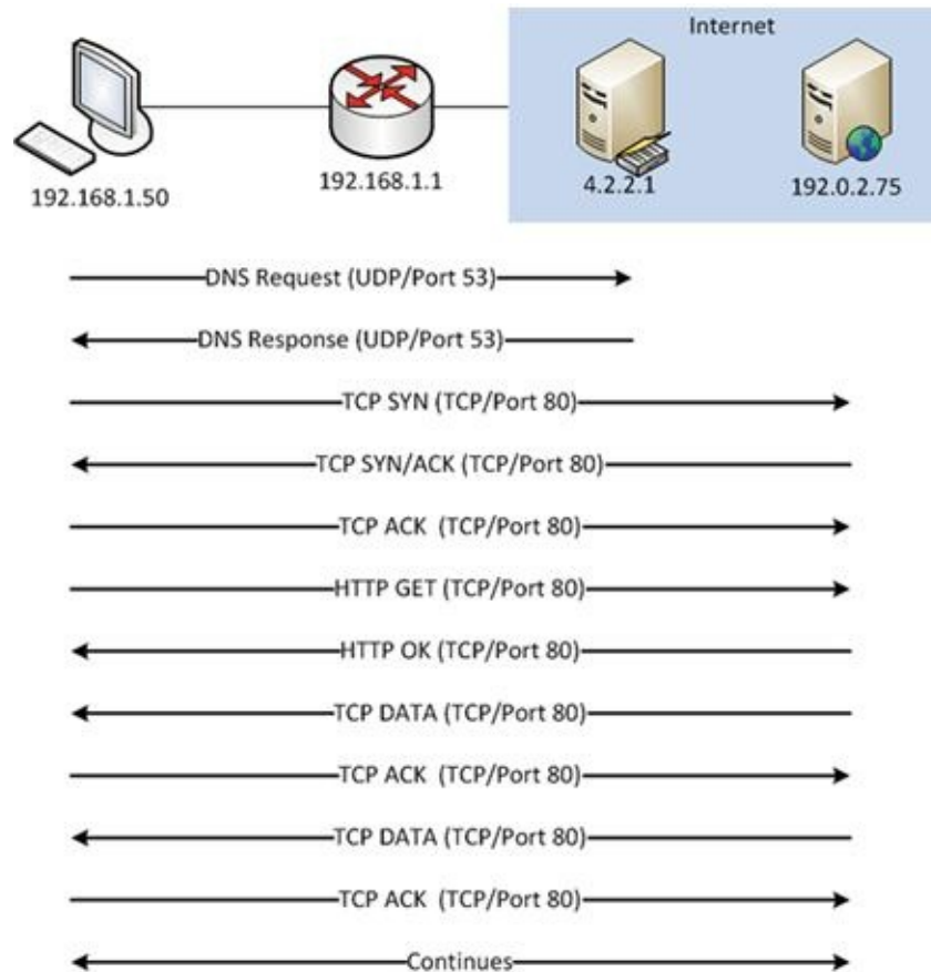
FIGURE 4.3 Web Server Communication Sequence
