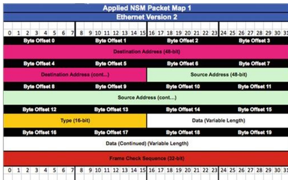
FIGURE 13.13 Packet Map for the Ethernet Header
