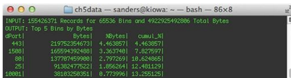
FIGURE 5.9 Top Communicating Destination Ports
