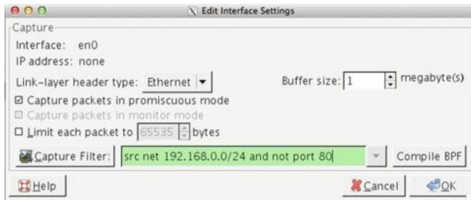
FIGURE 13.40 Specifying a Capture Filter
