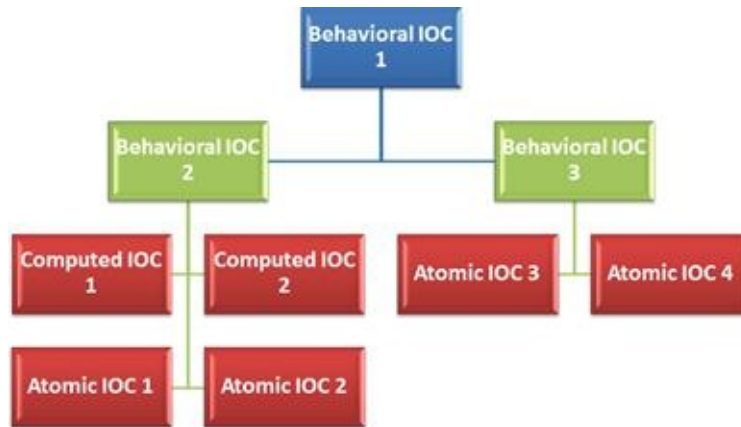
FIGURE 7.1 Atomic and Computed Indicators Comprise Behavioral Indicators
