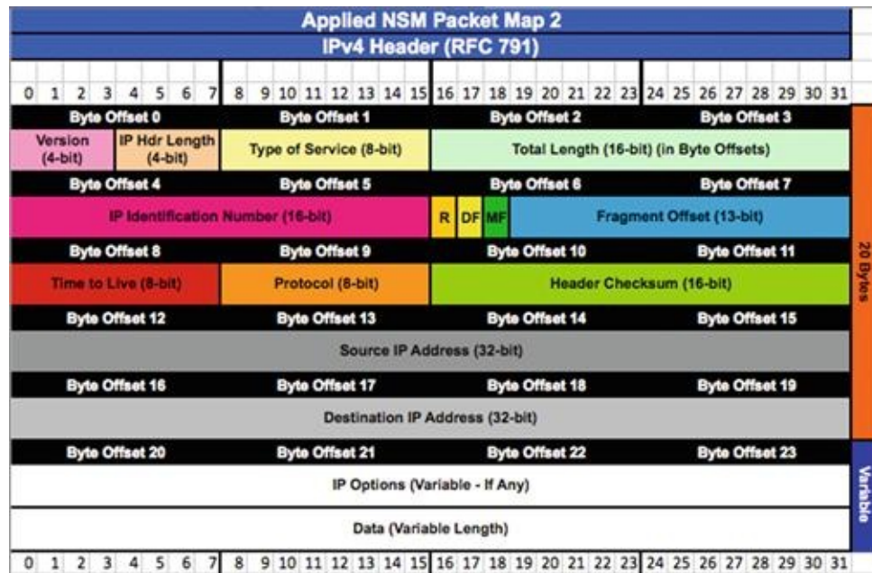
FIGURE 13.9 Packet Map for the IP Header
