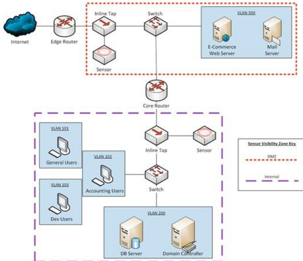
FIGURE 2.3 Updated Network Diagram Including Sensor Placement
