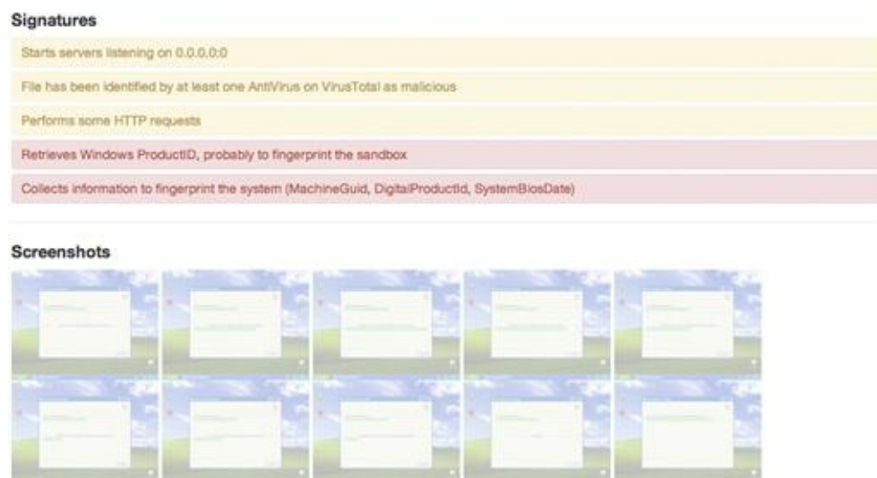
FIGURE 14.20 Cuckoo Report Showing Matching Signatures and Screenshots
