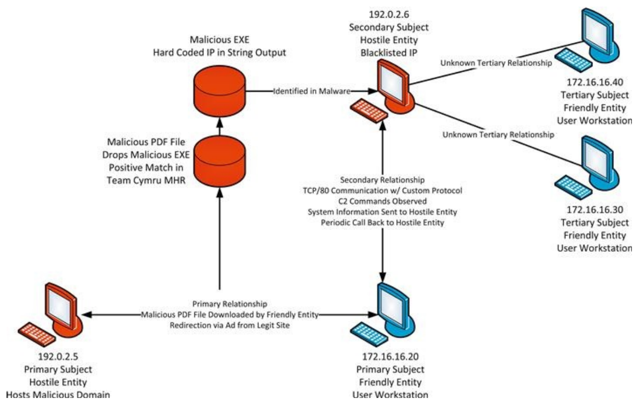
FIGURE 15.4 Relationship of Primary and Secondary Subjects
