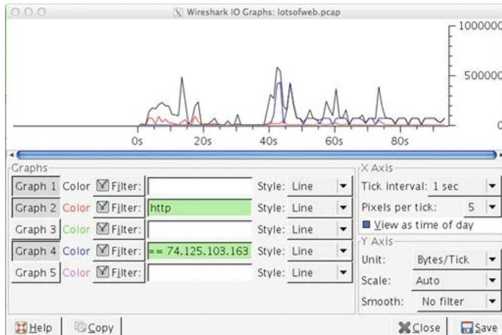
FIGURE 13.36 Viewing Capture Throughput with an IO Graph
