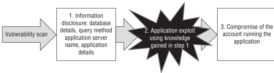
FIGURE 6.5 Exploit chaining
