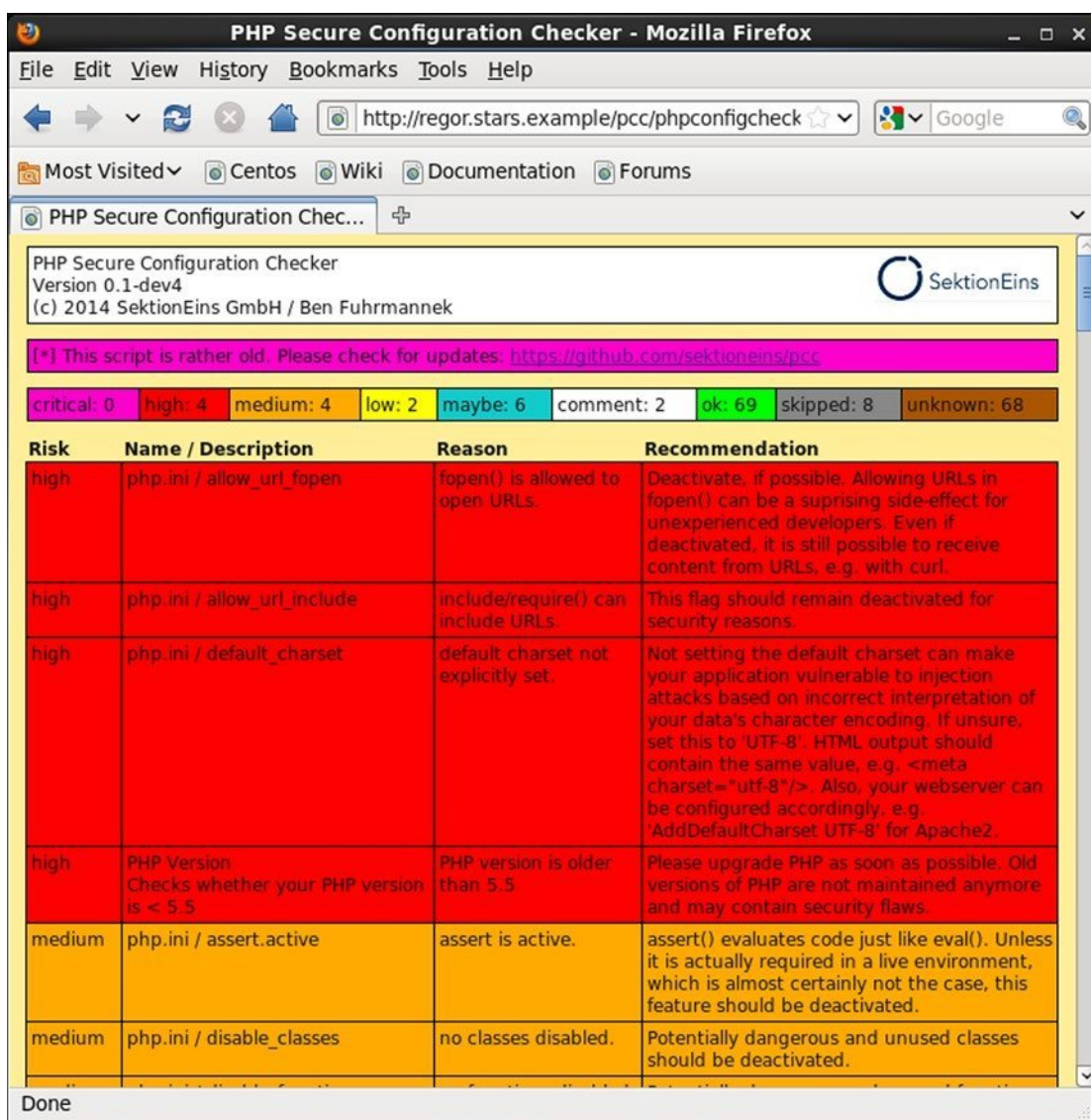
Figure 17-10. PHP Secure Configuration Checker run on a CentOS 6.1 system with allow_url_include set to On
