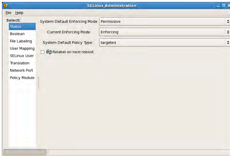
Figure 9-1. The system-config-selinux status screen
