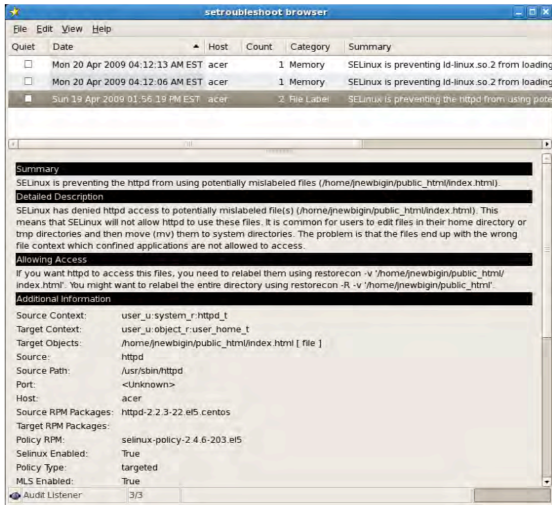
Figure 9-3. Explanation from SELinux Troubleshooter
