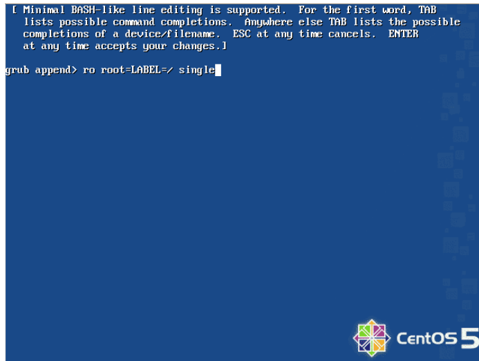
Figure 19-8. The parameter you add to enter single-user mode
