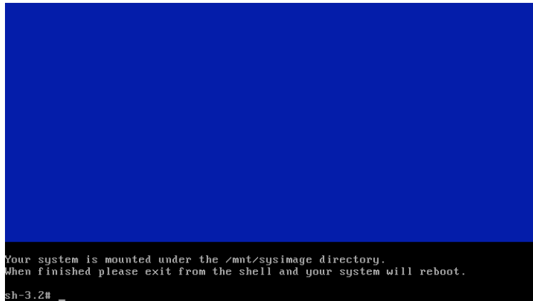
Figure 19-4. The rescue environment shell prompt
