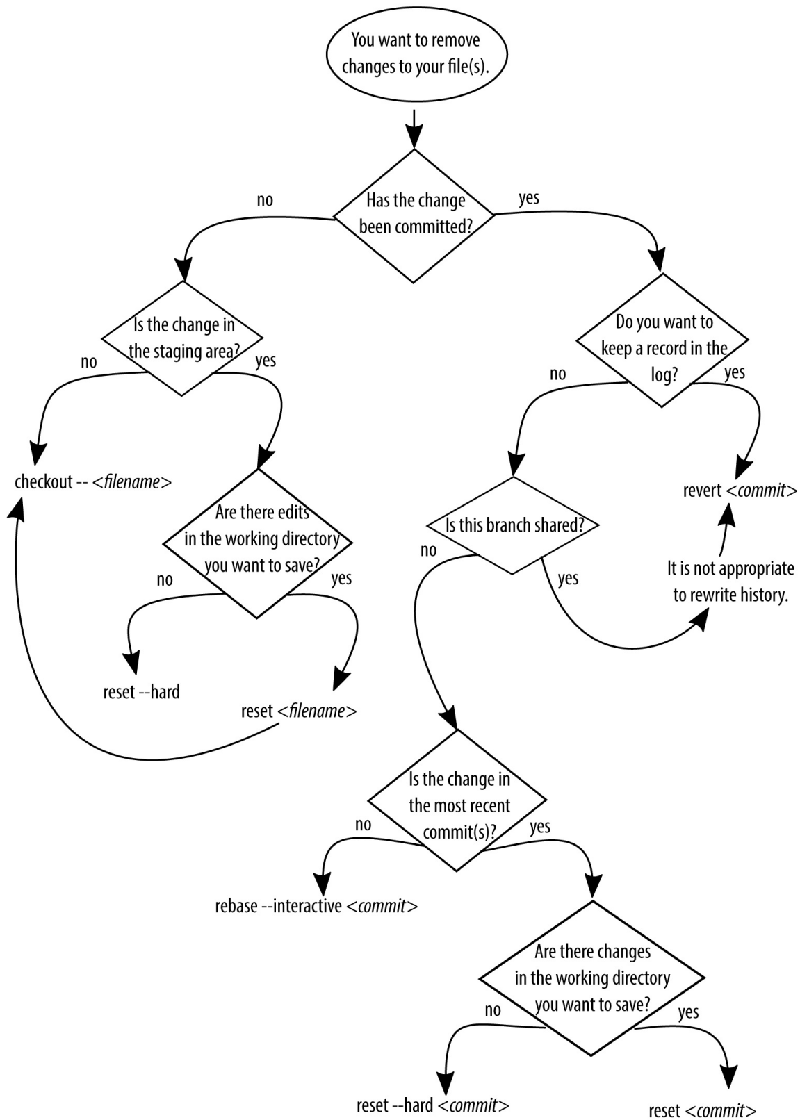
Figure 6-3. Create a flowchart to help you select the appropriate command
