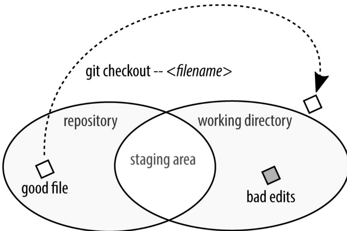
Figure 6-2. You want to discard changes you’ve made to a file in your working directory; the incorrect copy of the file is not staged or committed
