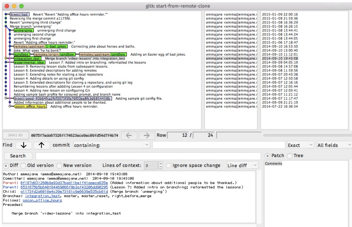
Figure 9-3. Running git bisect visualize shows you the current status of the bisect process
