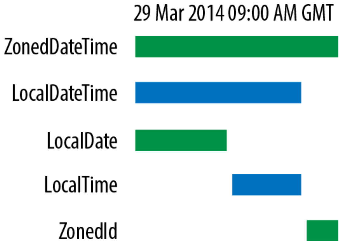
Figure 9-1. Breaking apart a timestamp
