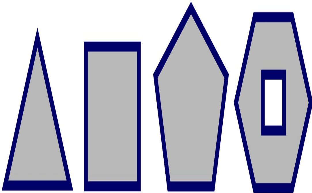
Figure 15-8. Regular polygons
