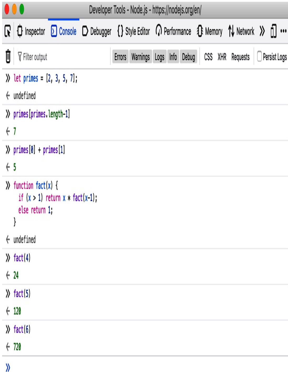
Figure 1-1. The JavaScript console in Firefox's Developer Tools
