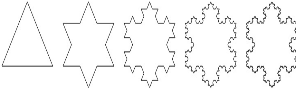
Figure 15-12. Koch snowflakes
