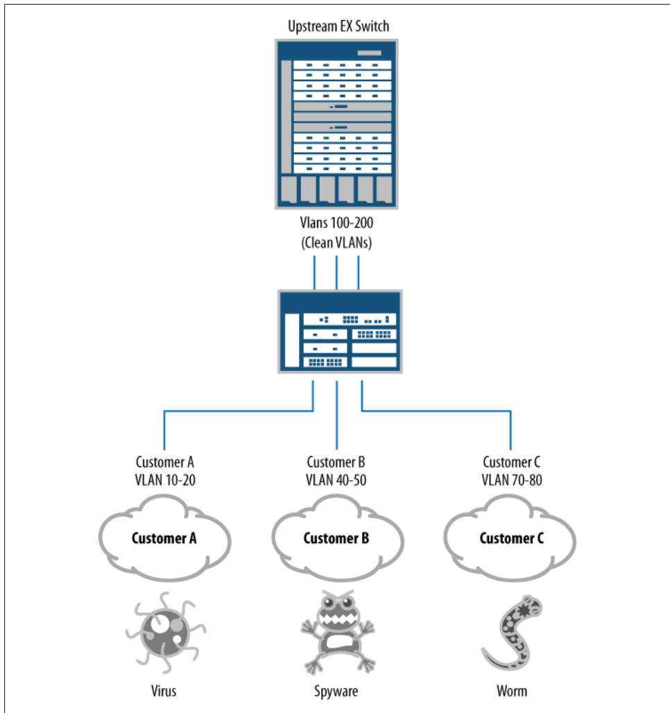
Figure 12-2. VLAN rewriting
