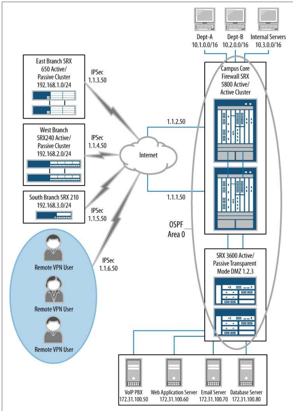
Figure 11-6. Organization-XYZ's OSPF routing topology
