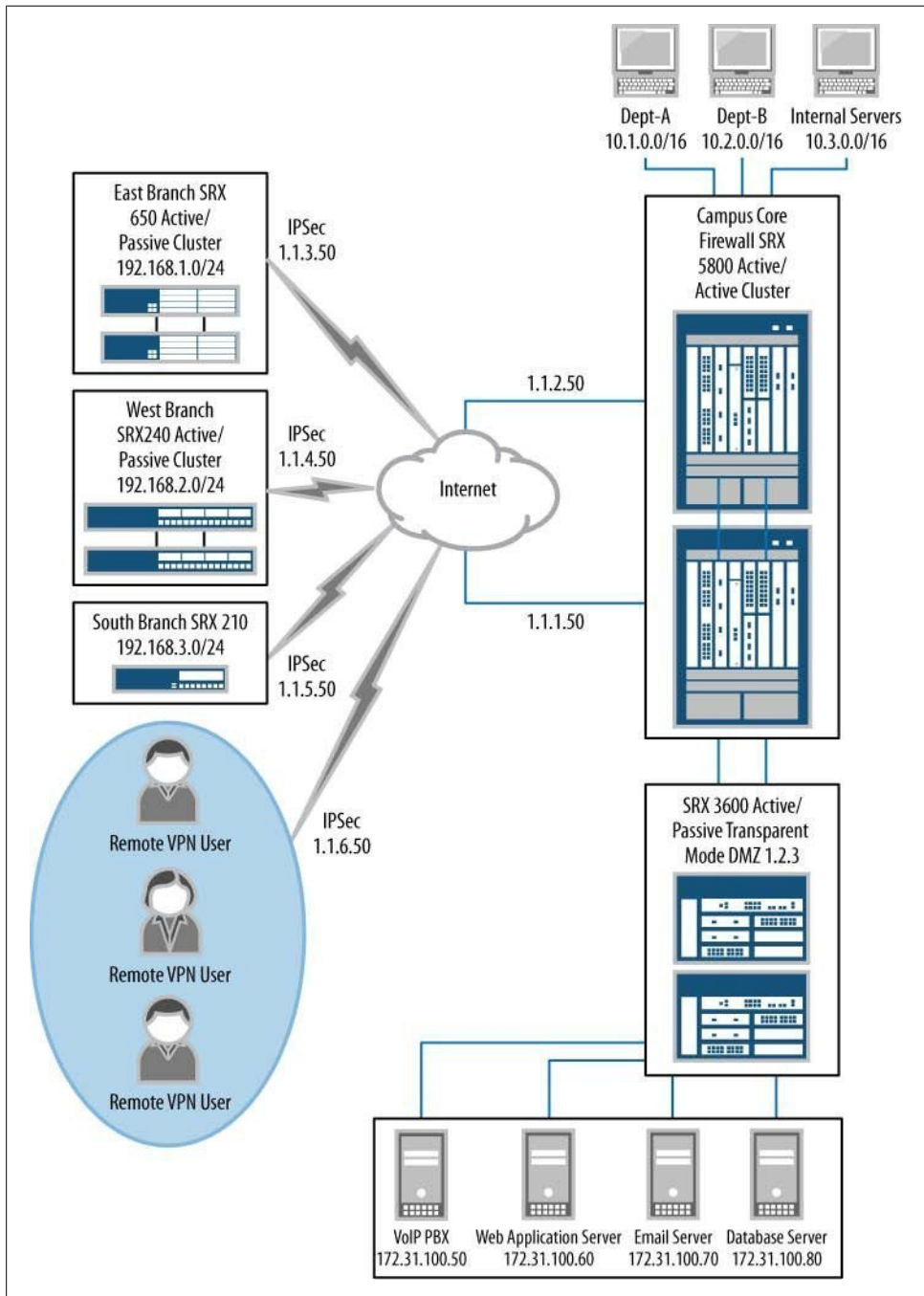
Figure P-1. This book's topology
