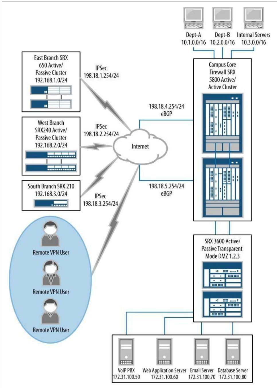
Figure 6-6. IPsec VPN infrastructure
