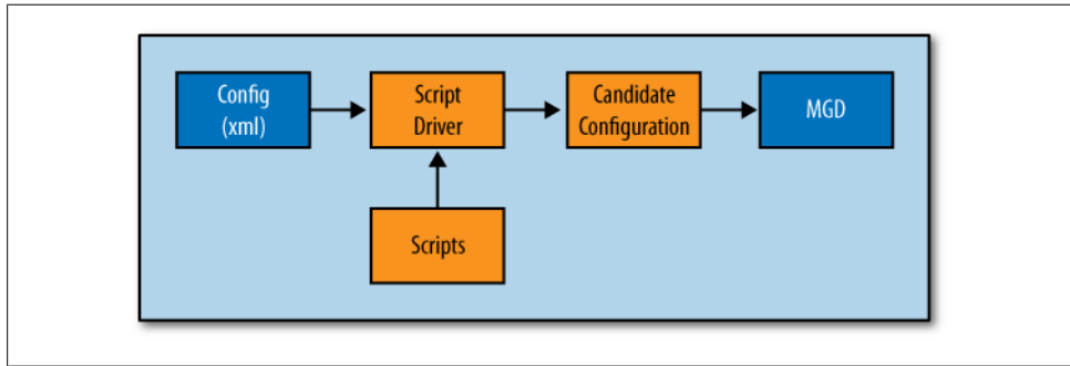
Figure 13-4. Commit scripts
