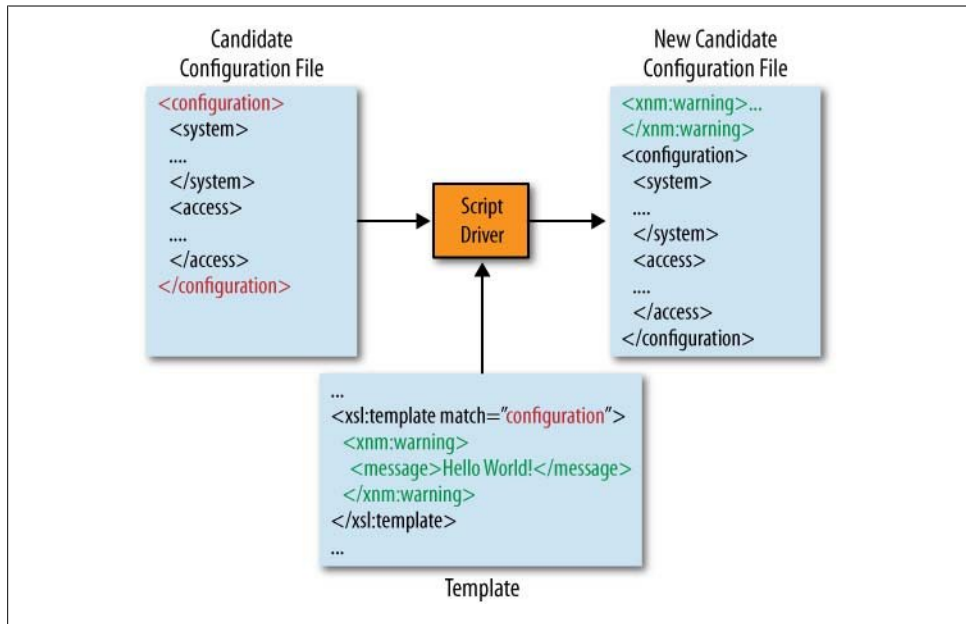
Figure 13-5. Template processing
