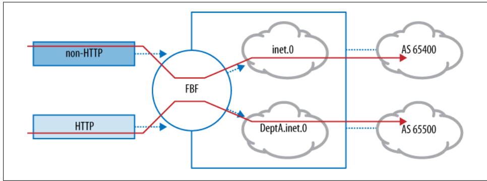
Figure 11-12. Filter-based forwarding
