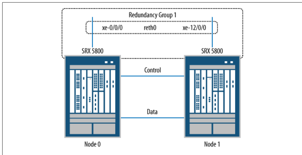
Figure 10-4. Reth example
