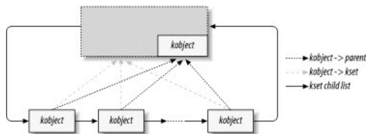
Figure 14-2. A simple kset hierarchy
