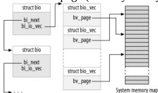
Figure 16-1. The bio structure
