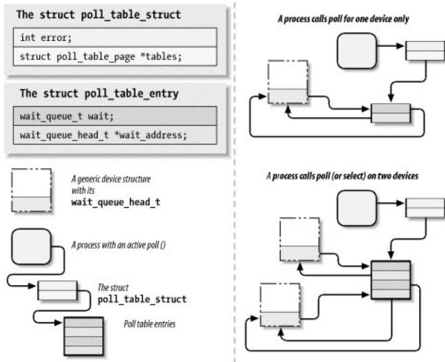
Figure 6-1. The data structures behind poll
