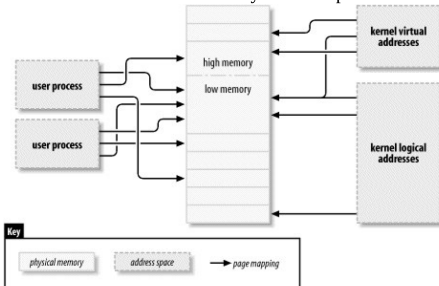
Figure 15-1. Address types used in Linux
