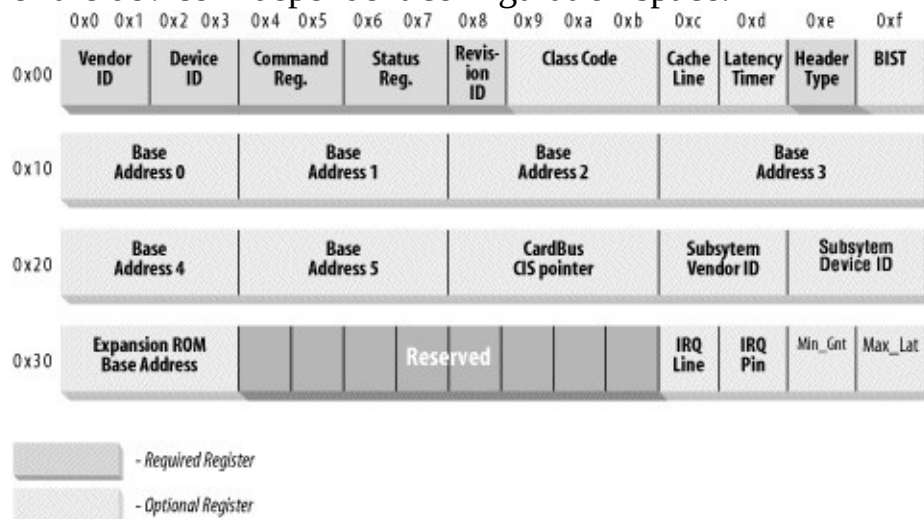
Figure 12-2. The standardized PCI configuration registers
