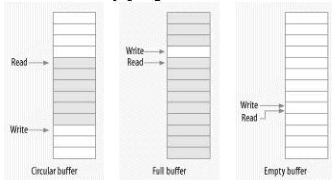
Figure 5-1. A circular buffer
