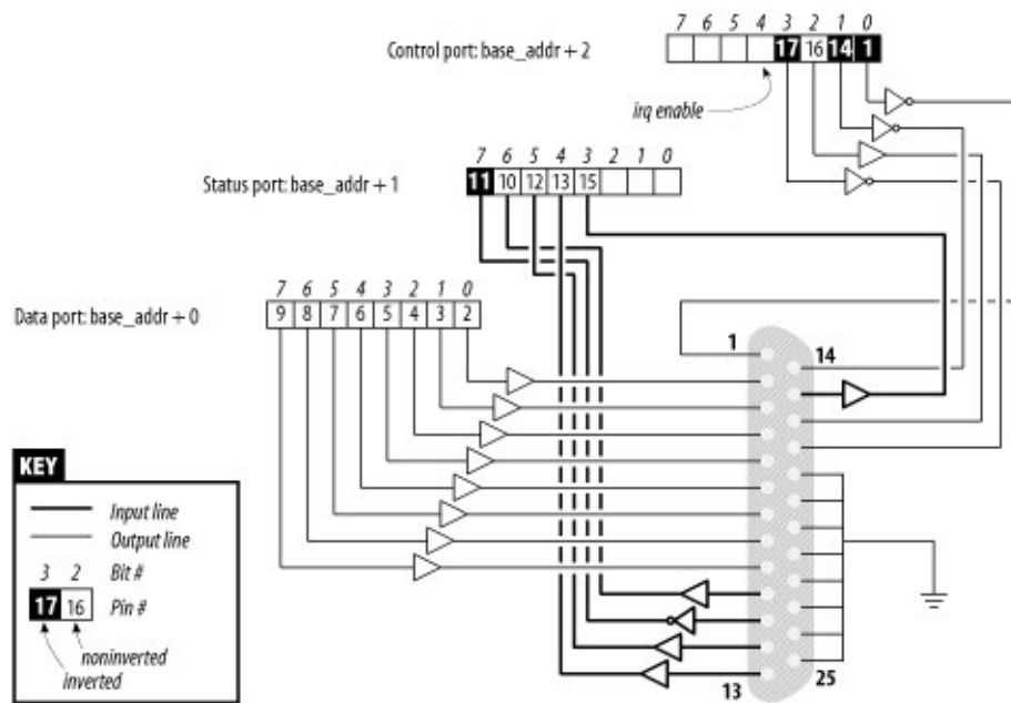
Figure 9-1. The pinout of the parallel port
