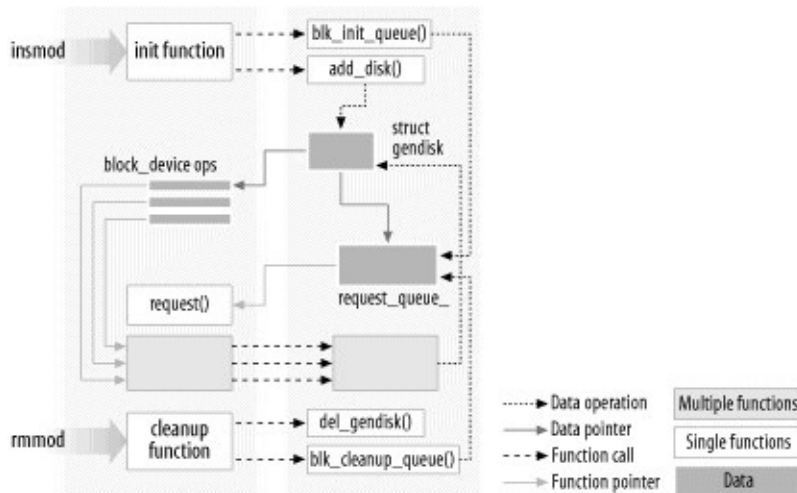
Figure 2-1. Linking a module to the kernel
