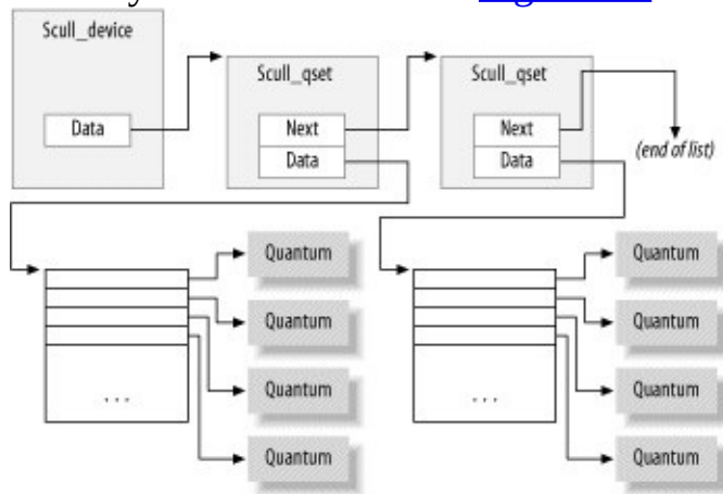
Figure 3-1. The layout of a scull device
