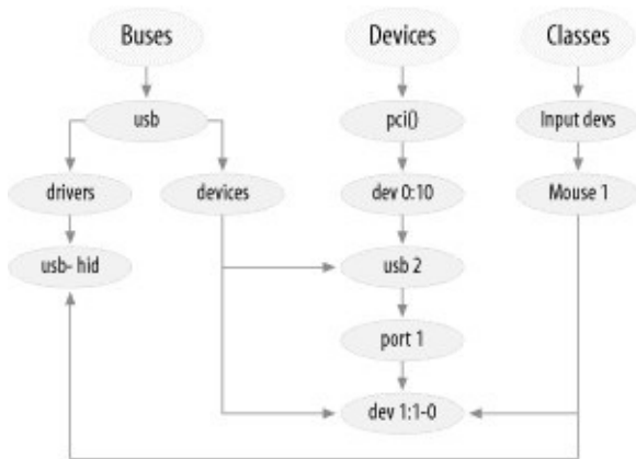
Figure 14-1. A small piece of the device model
