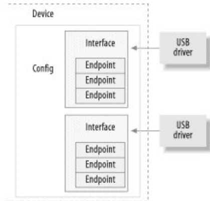
Figure 13-2. USB device overview
