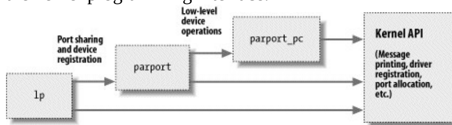
Figure 2-2. Stacking of parallel port driver modules
