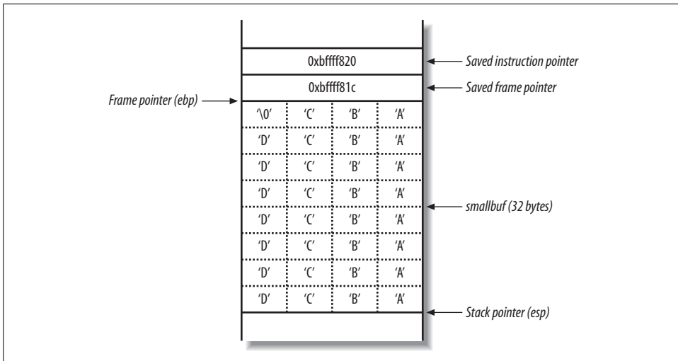
Figure 14-8. The vulfunc() stack frame with 31 characters
