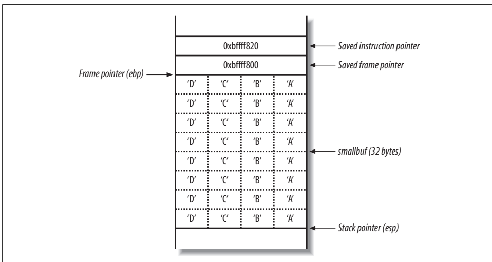
Figure 14-9. The vulfunc() stack frame with 32 characters
