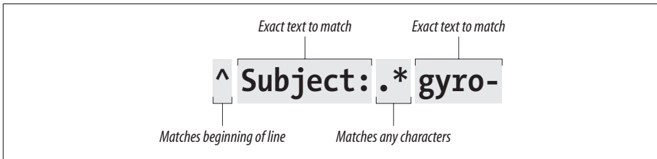
Figure 19-25. Simple regular expression
