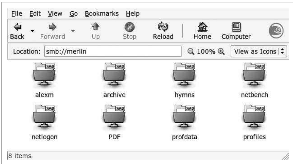
Figure 15-2. GNOME File Manager using the libsmbclient module
