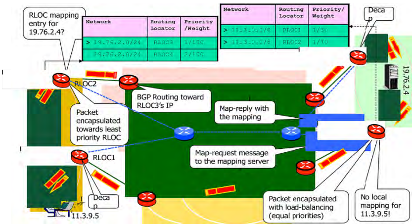
Figure 4.12. LISP protocol
