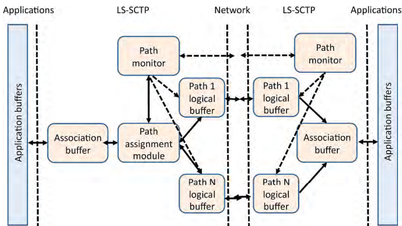
Figure 5.22. Architecture of LS-SCTP
