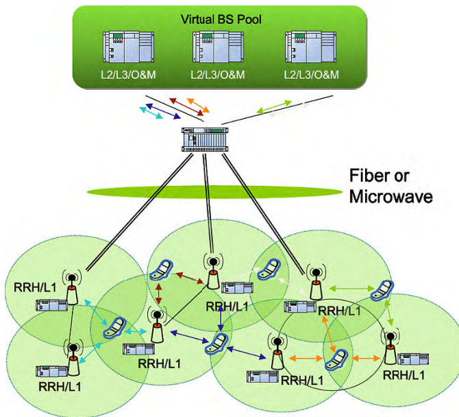
Figure 6.18. The partially-distributed Cloud-RAN architecture
