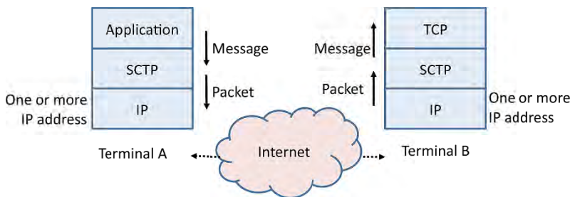
Figure 5.19. SCTP architecture
