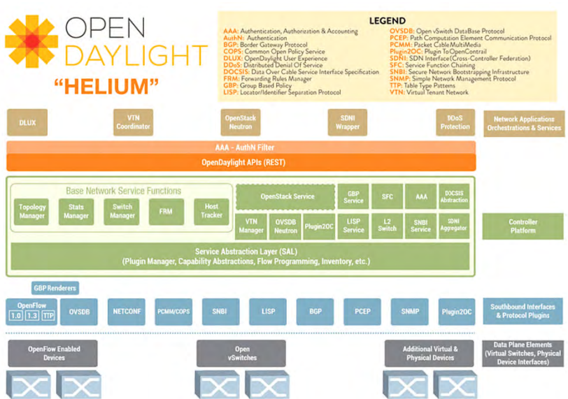
Figure 4.6. OpenDaylight controller
