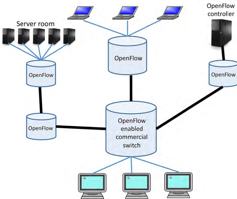
Figure 4.3. OpenFlow protocol in a network
