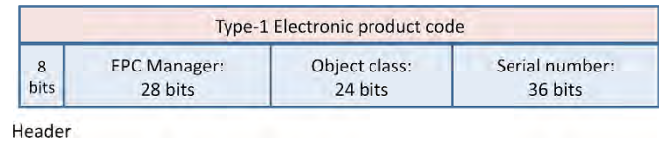
Figure 6.21. Structure of GEN1 Electronic Product Code
