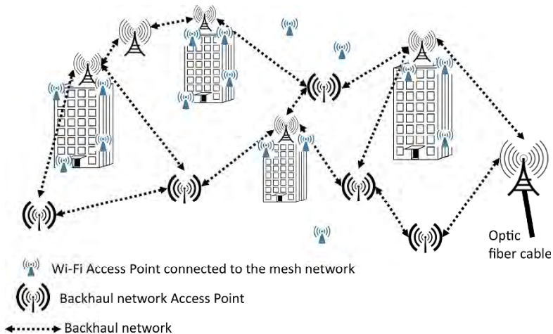
Figure 6.4. Small cells and backhaul networks
