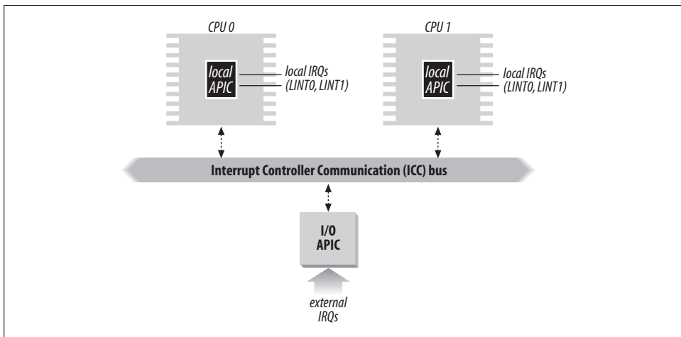
Figure 4-1. Multi-APIC system
