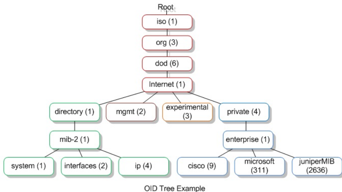
Figure 3-1. A simplified diagram showing the organization of nodes in an object identifier (OID) tree
