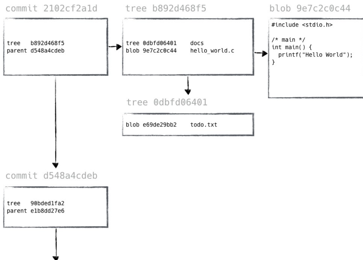
Figure 7-2. Git's database makes unwanted changes difficult, since objects are referenced using a hash of their contents
