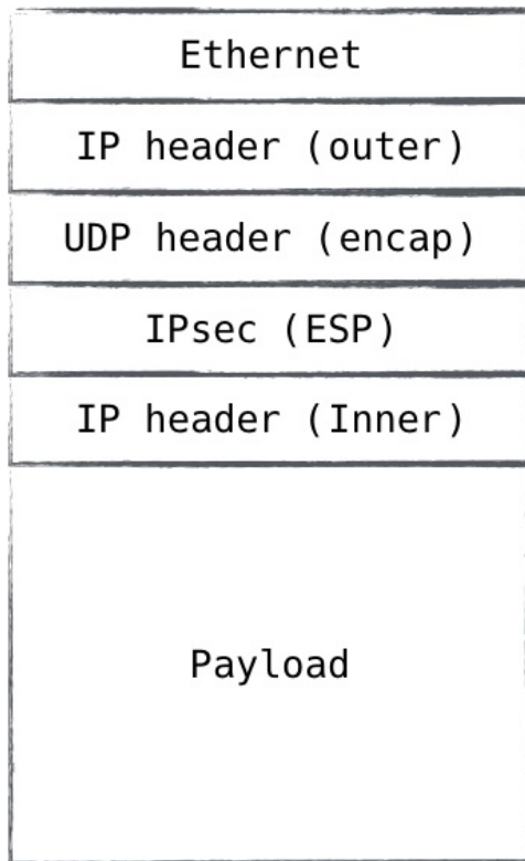
Tunnel mode
