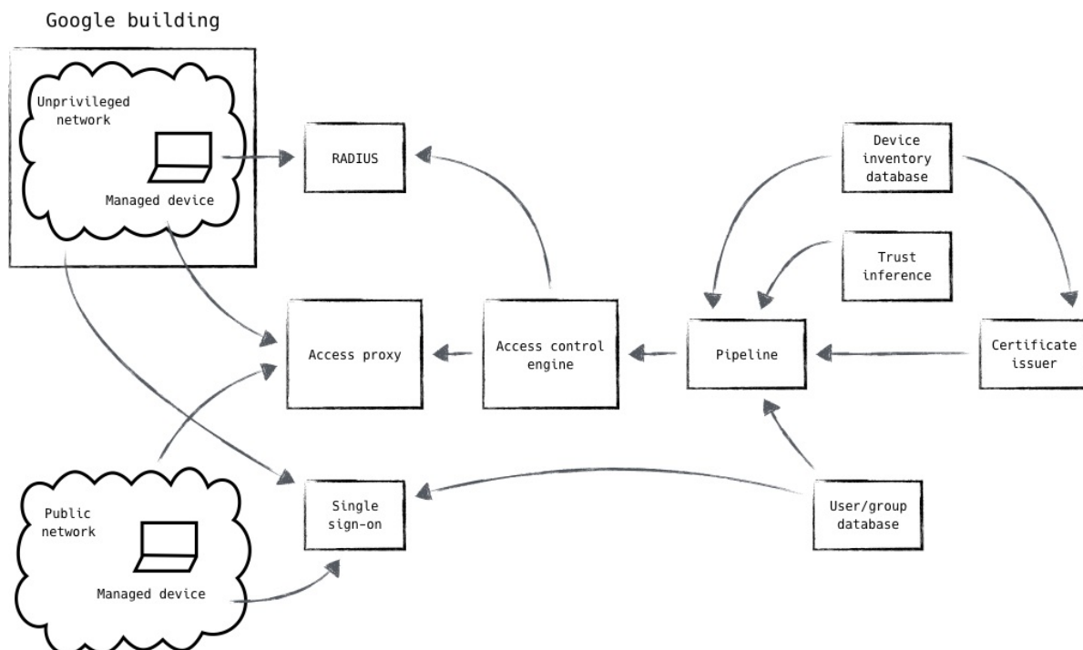
Figure 9-5. BeyondCorp components and access flow
